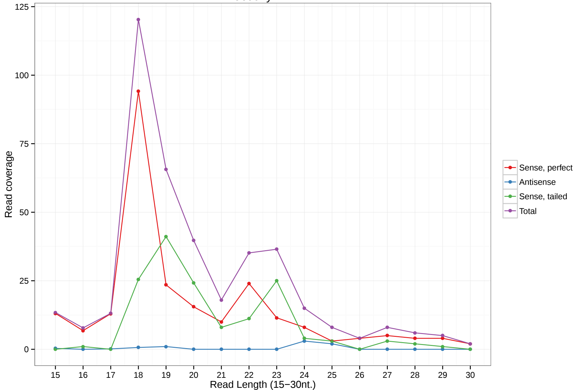
uc001ynf.4
