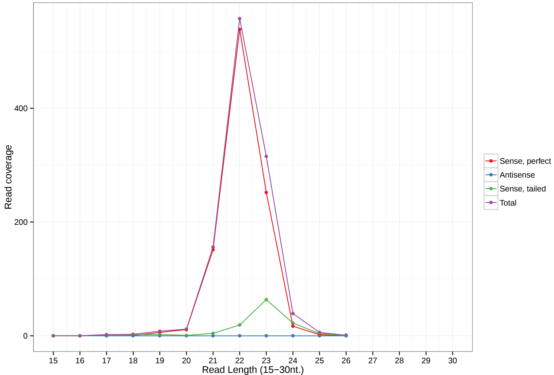
uc001xed.3
