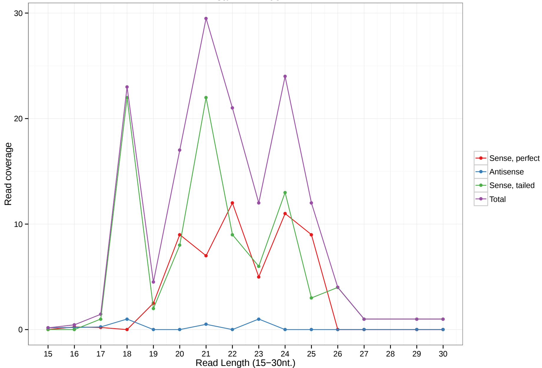
hsa-mir-7106
