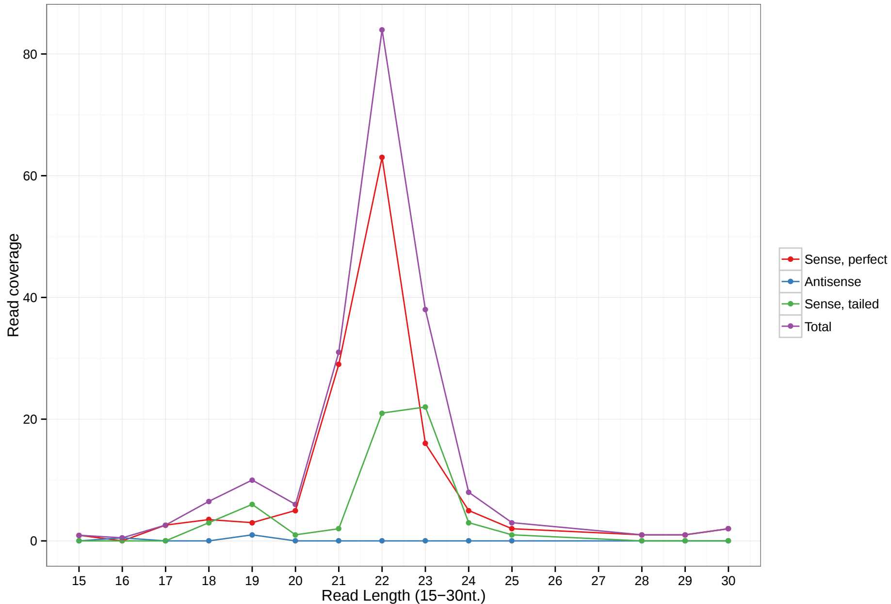
hsa-mir-6883
