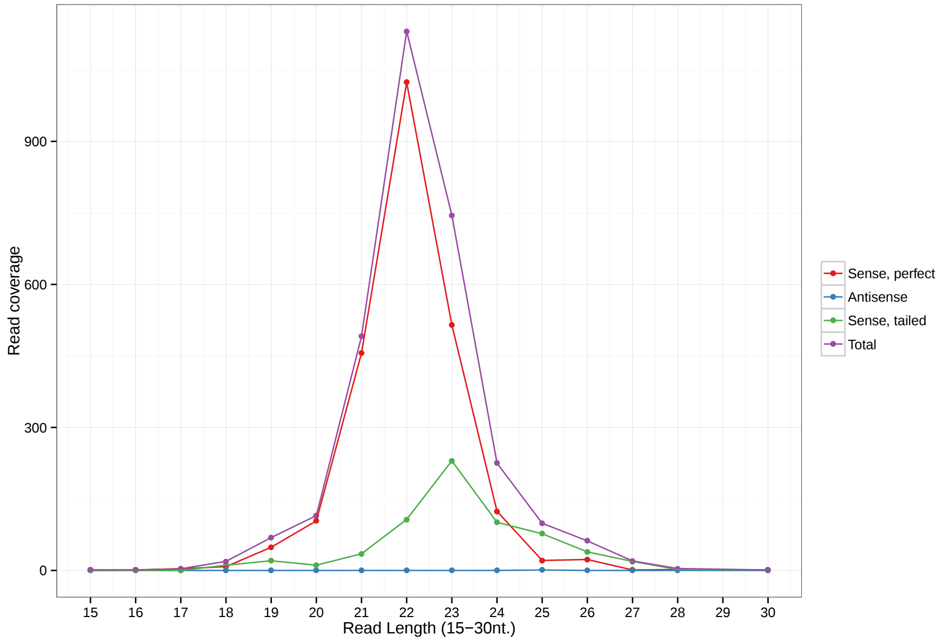
hsa-mir-6882
