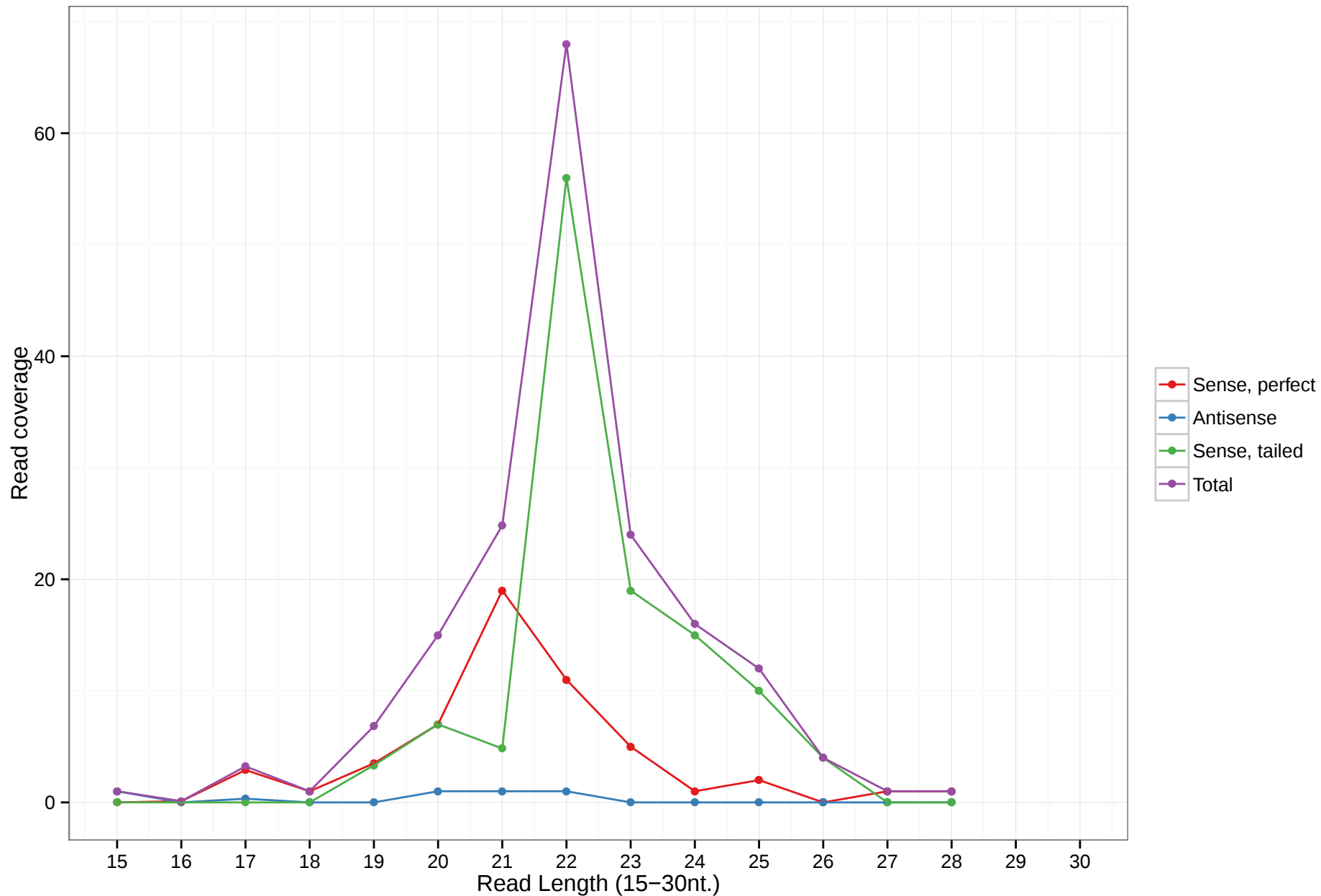
hsa-mir-6880
