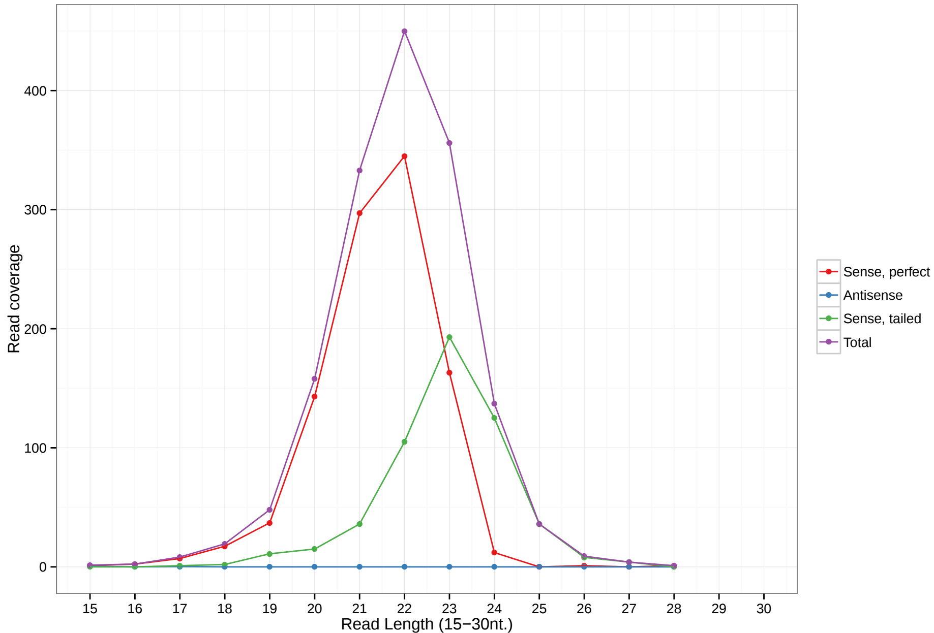
hsa-mir-6877
