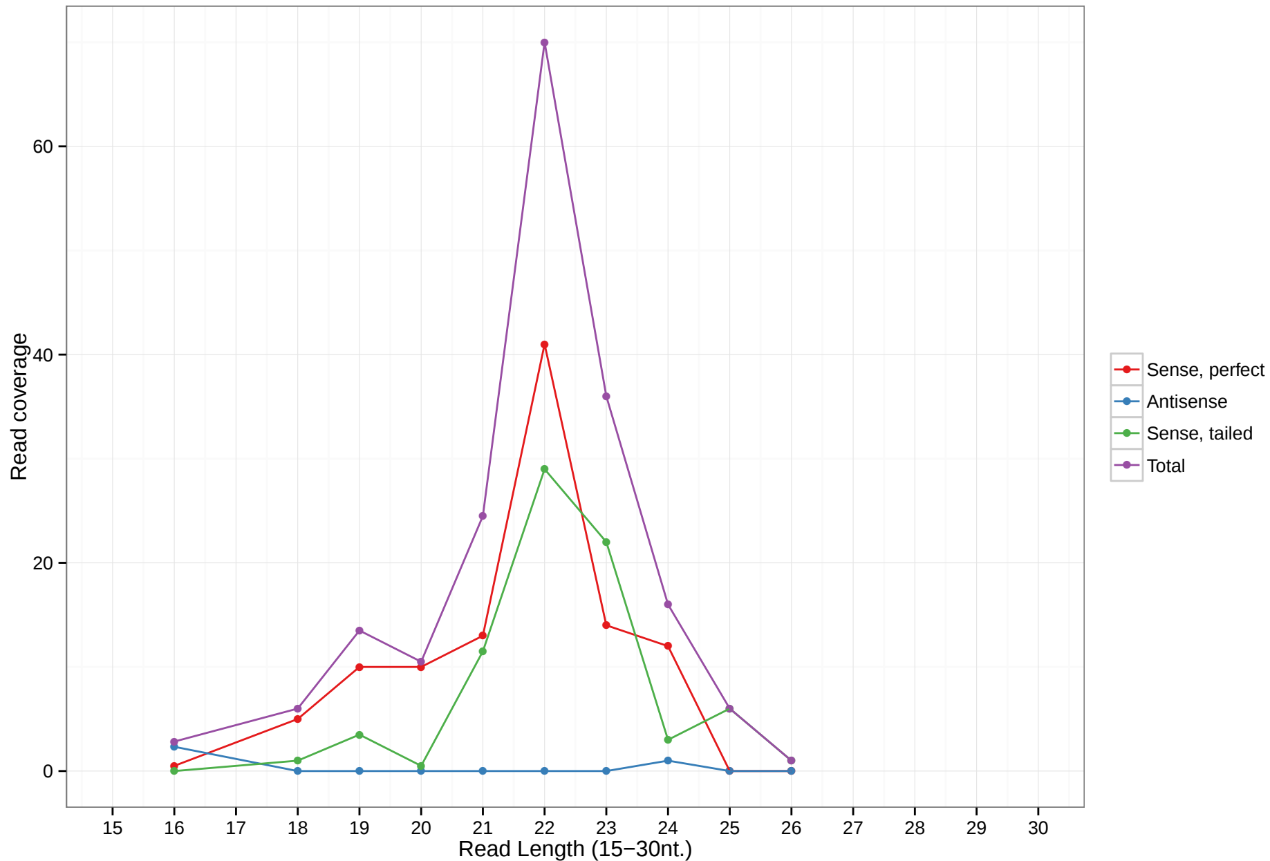
hsa-mir-6876
