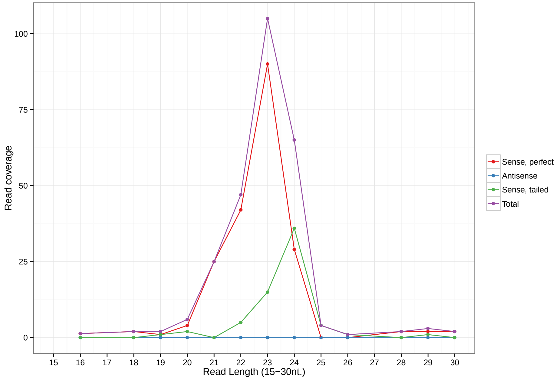
hsa-mir-6874
