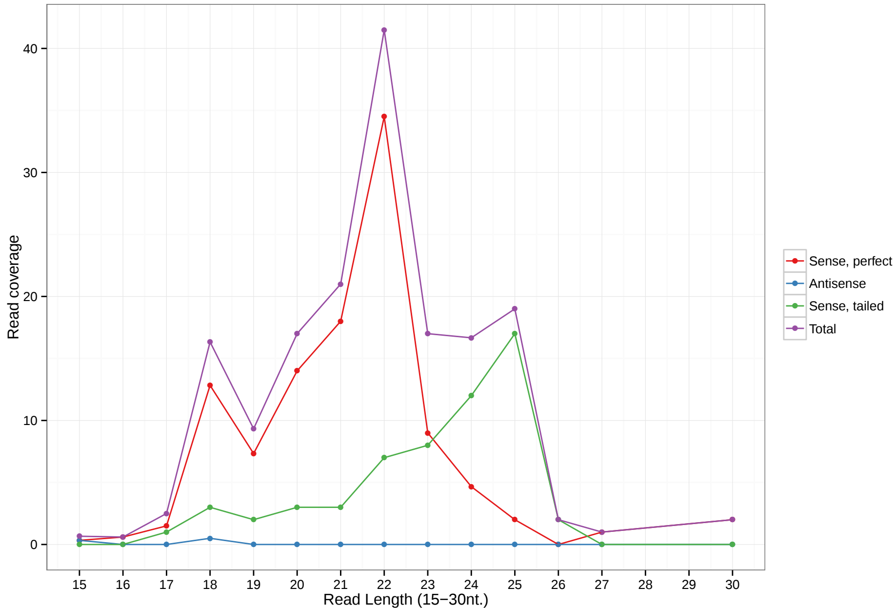
hsa-mir-6869
