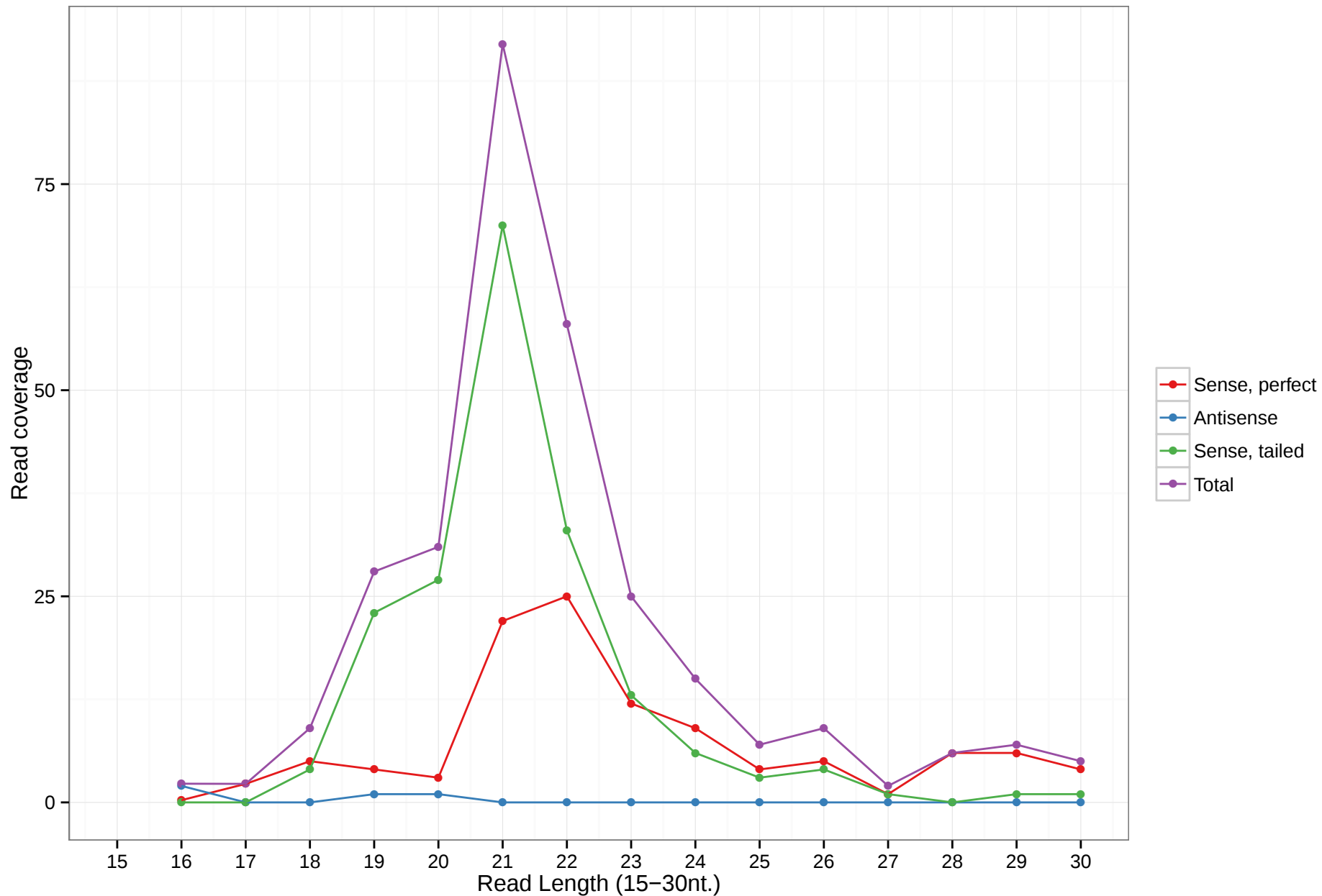
hsa-mir-6861
