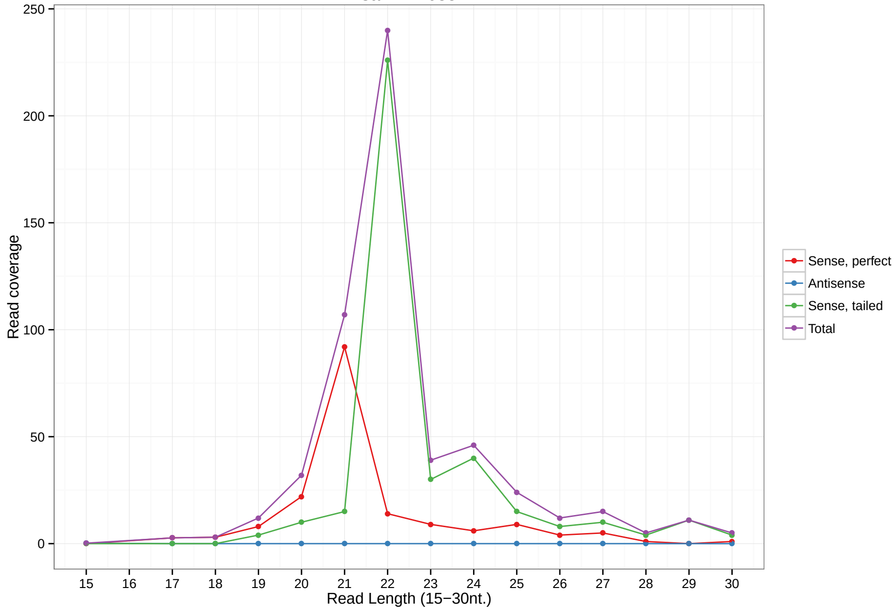
hsa-mir-6857
