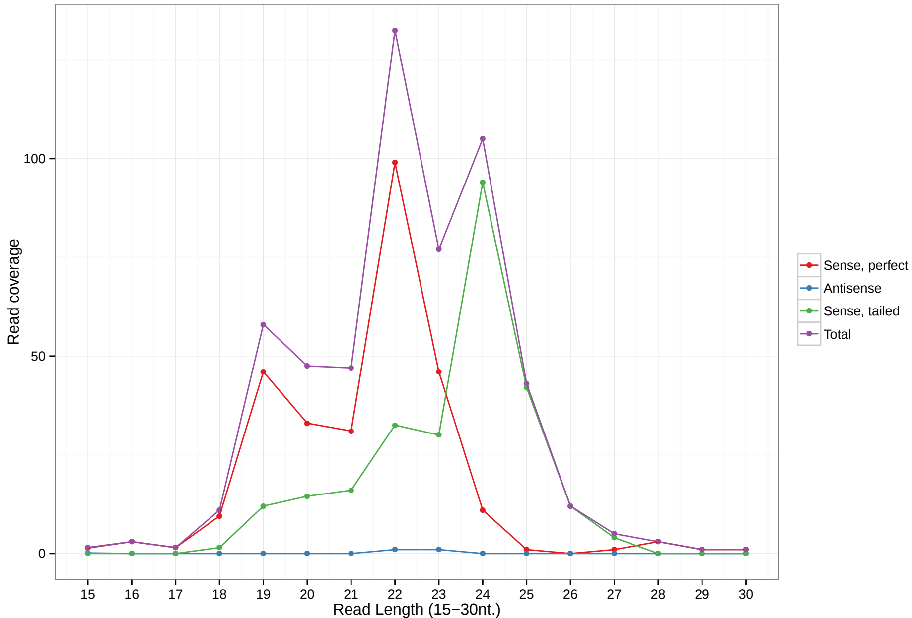
hsa-mir-6851
