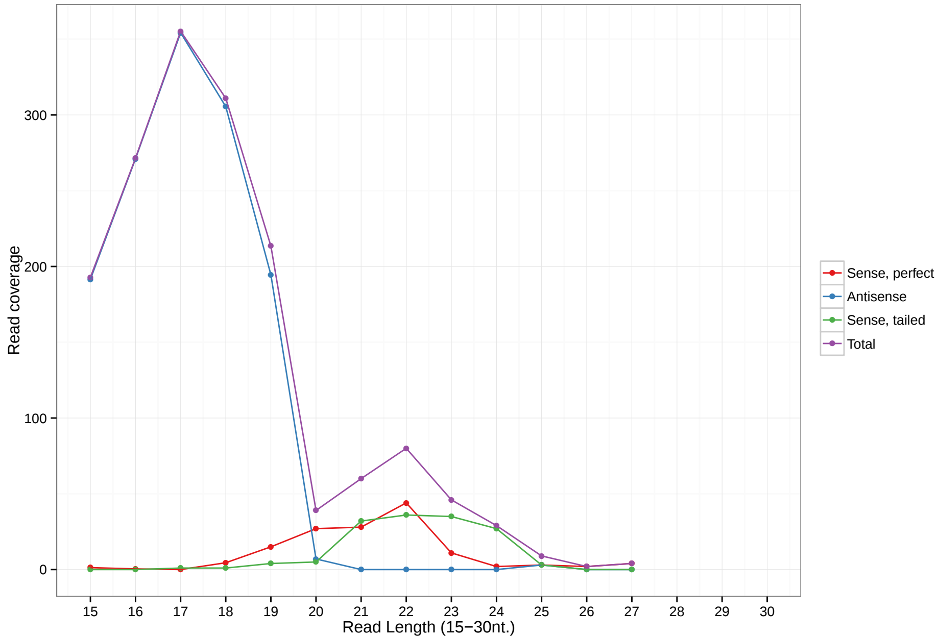
hsa-mir-6838
