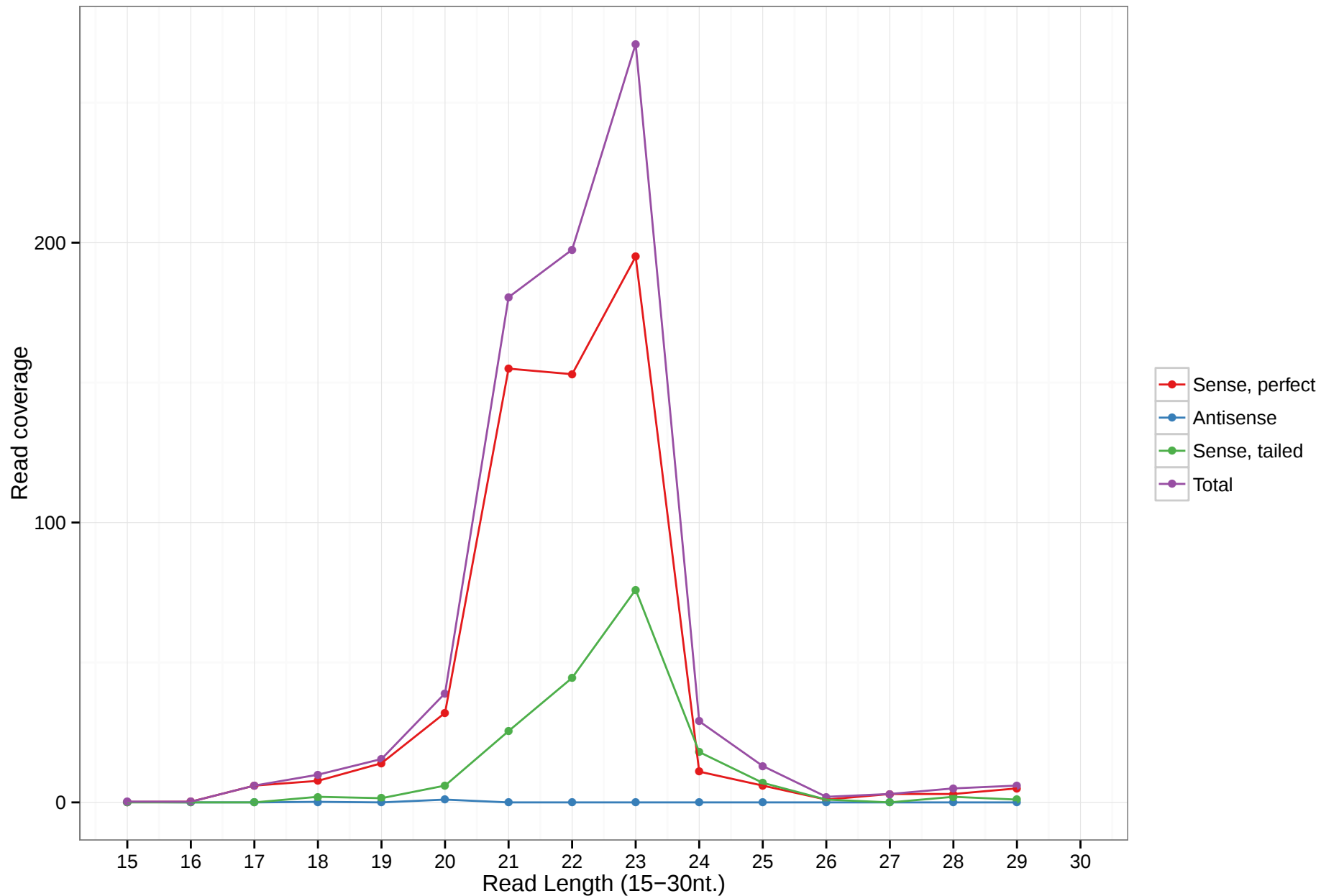
hsa-mir-6837
