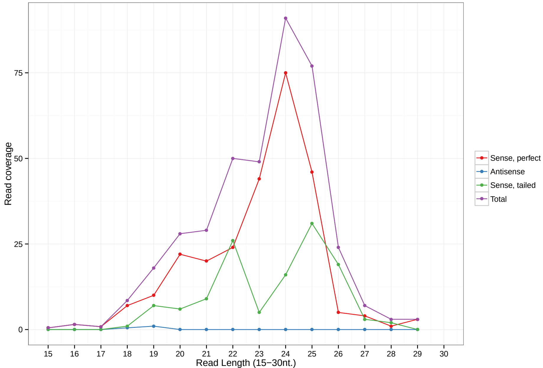
hsa-mir-6831
