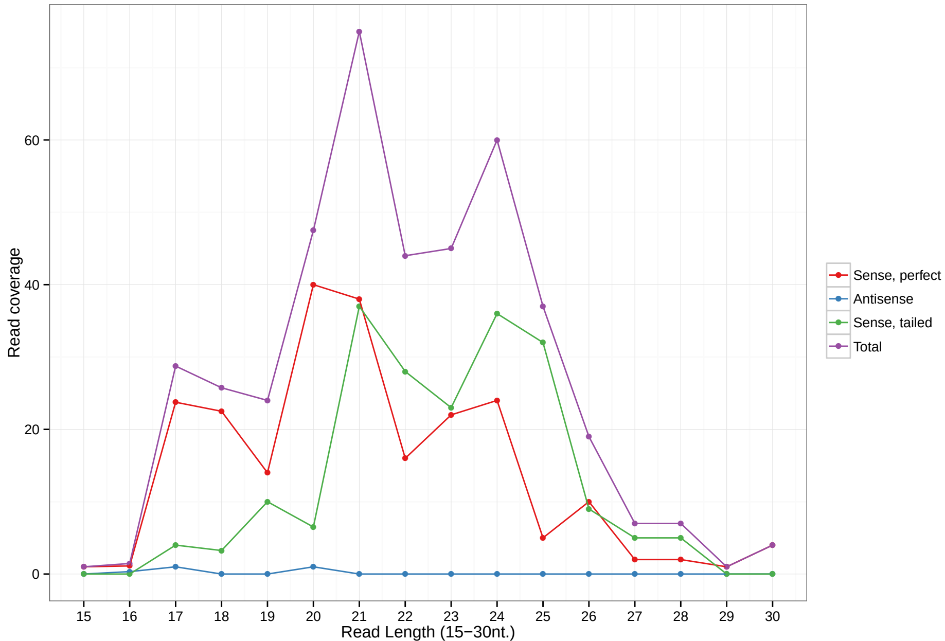
hsa-mir-6829
