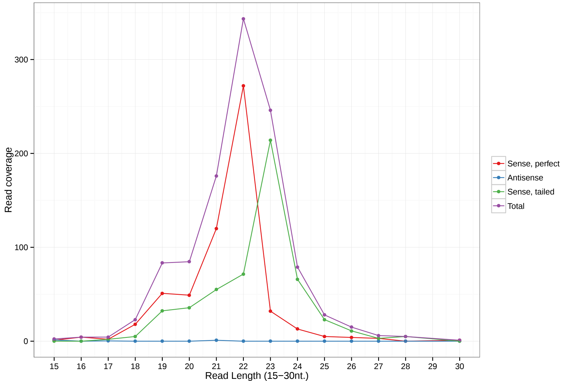
hsa-mir-6820
