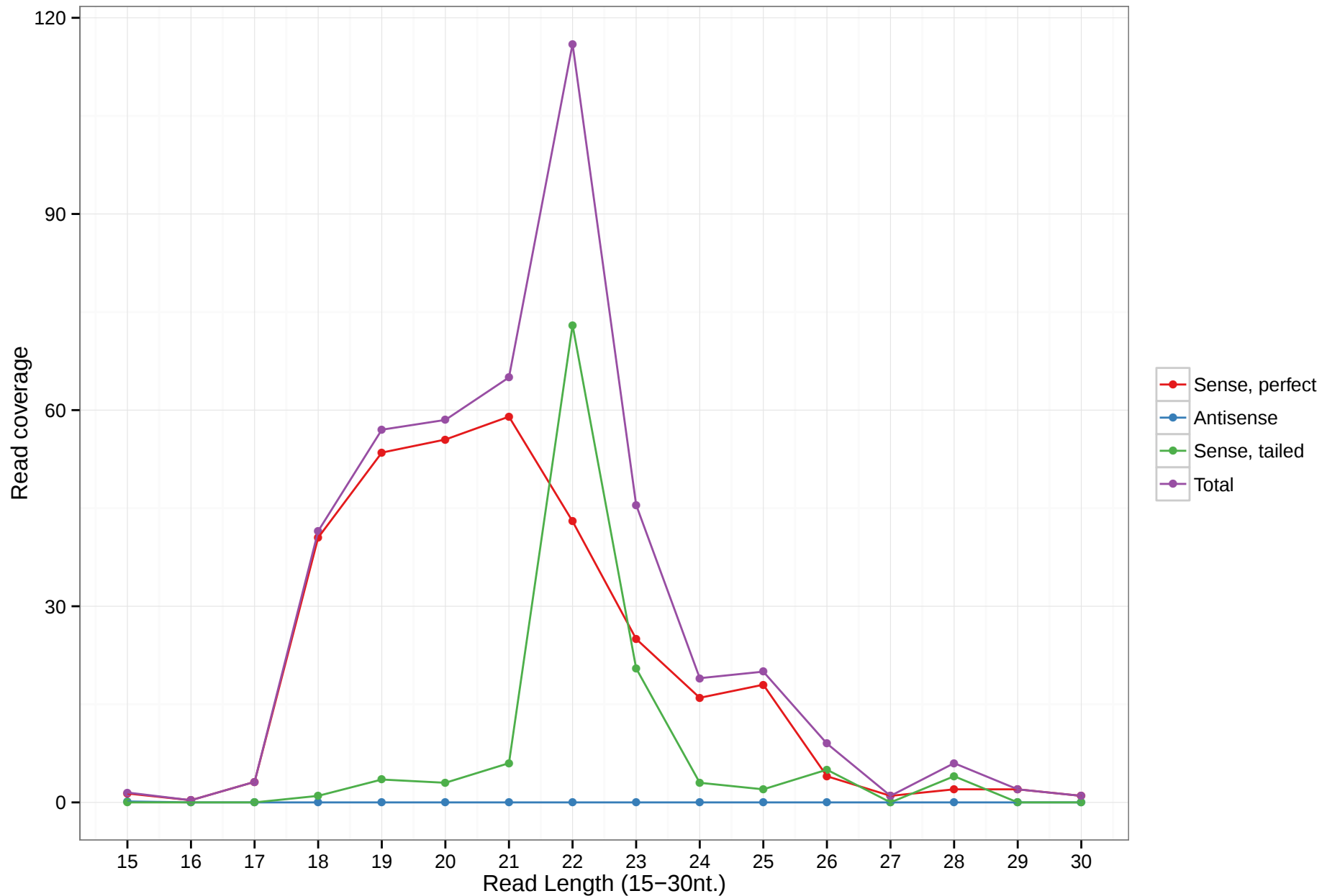
hsa-mir-6819
