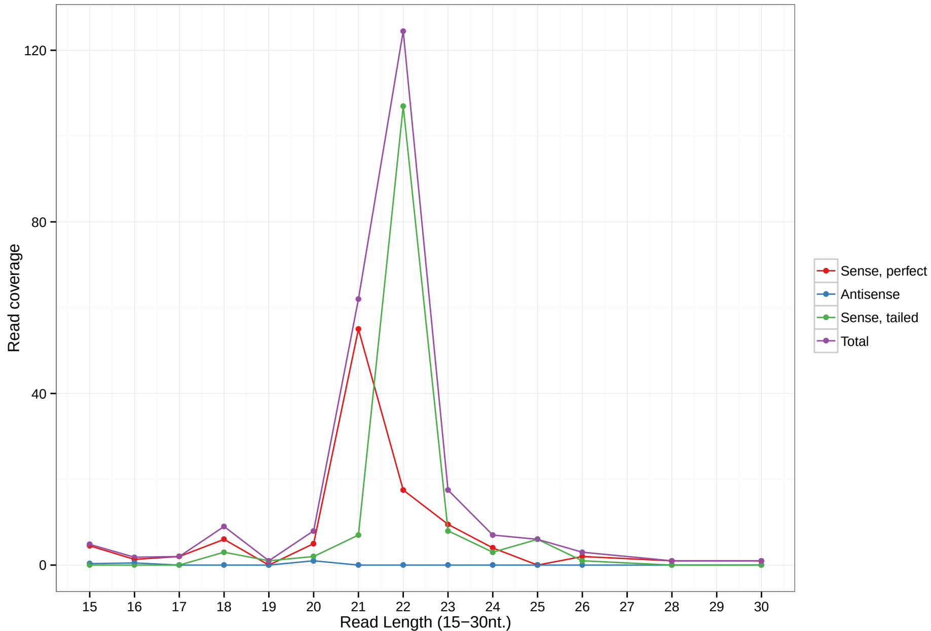
hsa-mir-6798
