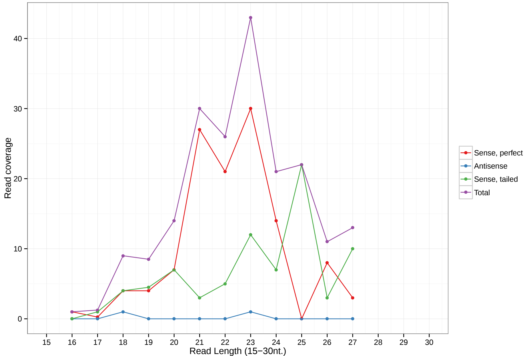
hsa-mir-6786
