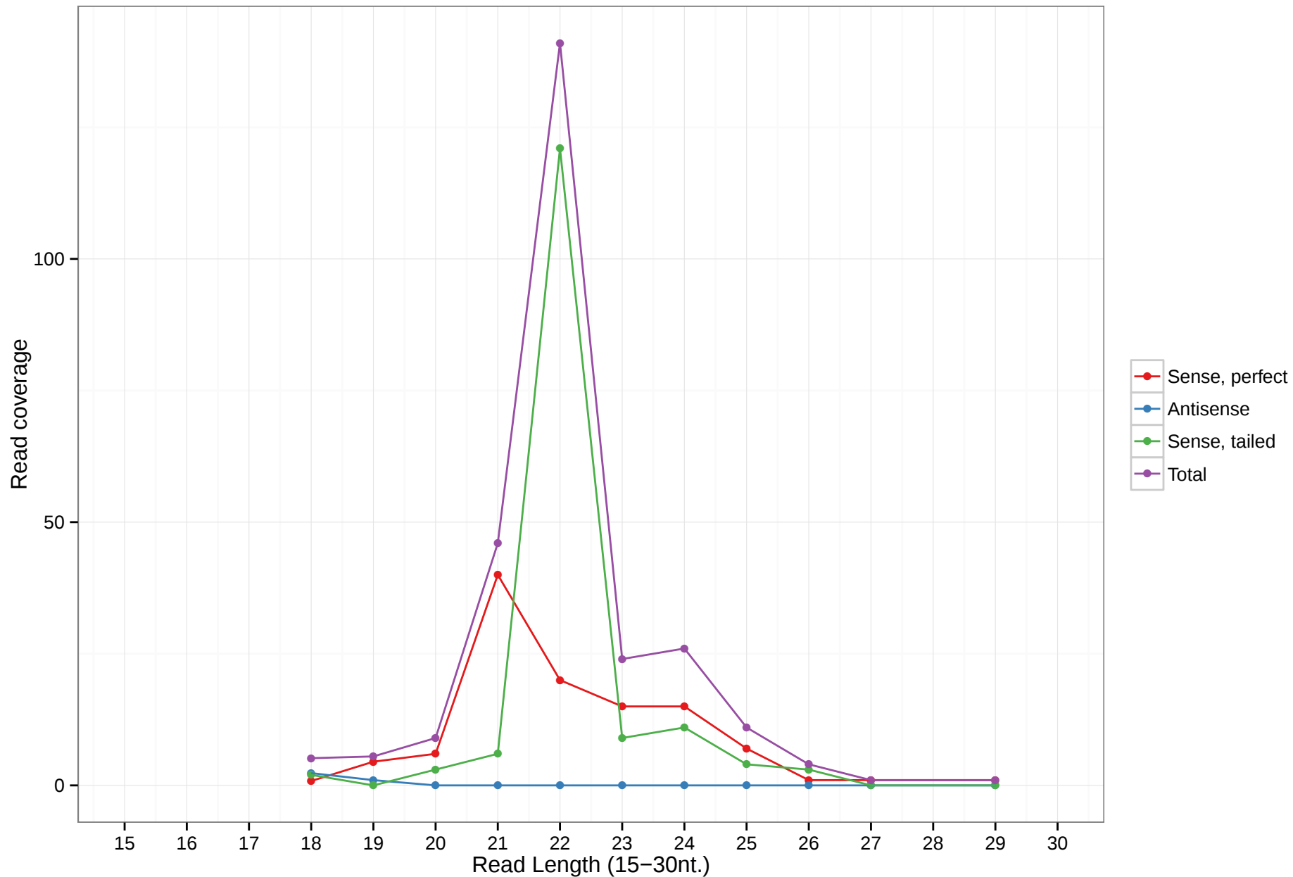
hsa-mir-6780b
