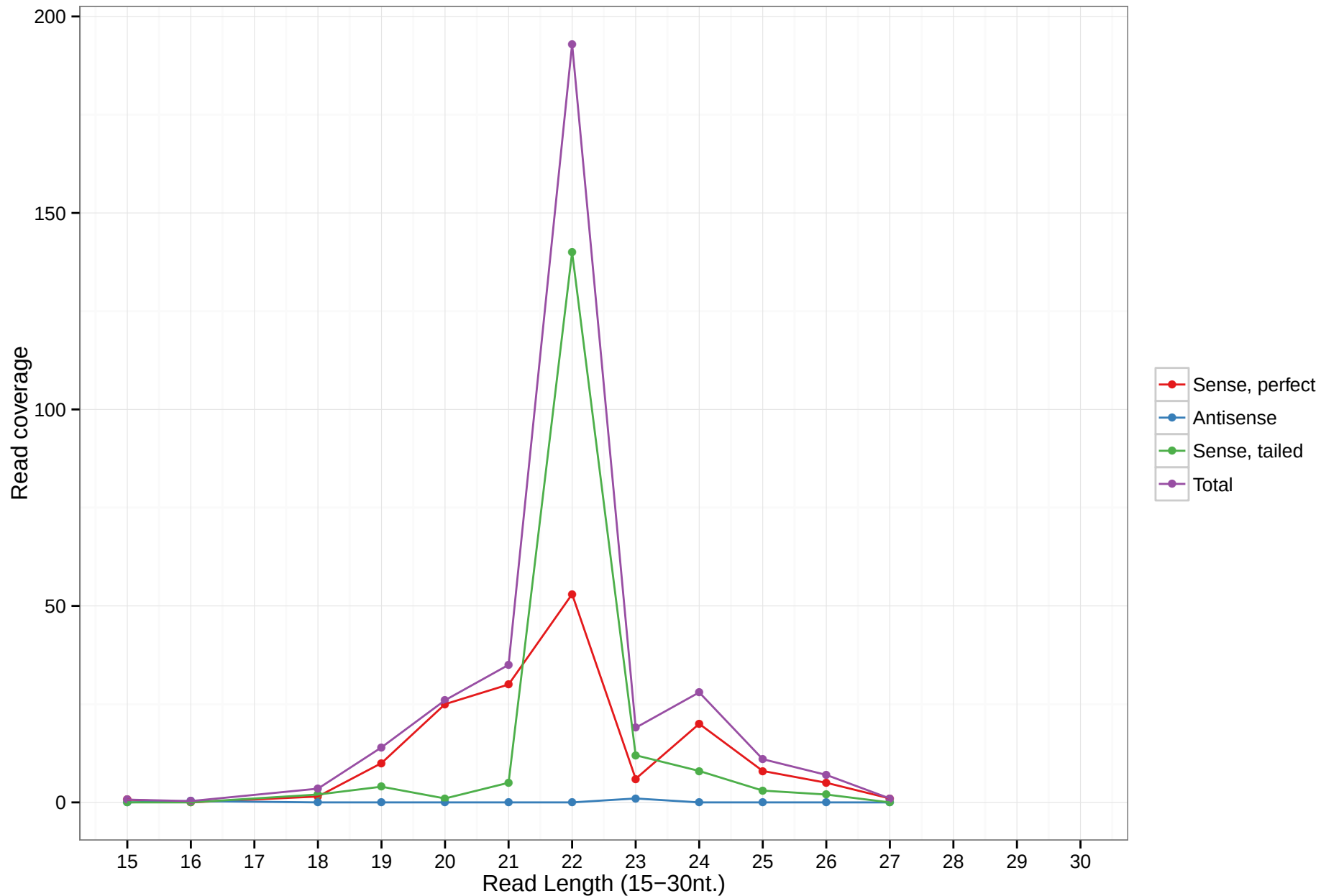
hsa-mir-6774
