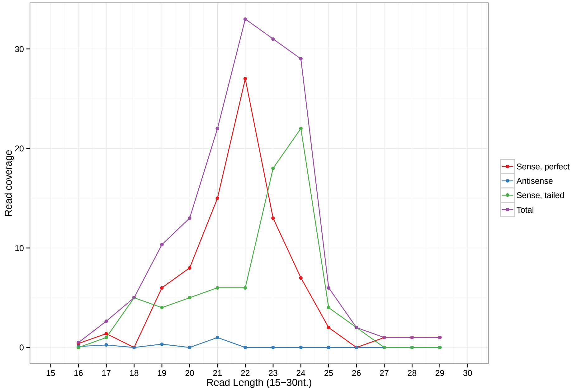
hsa-mir-6754
