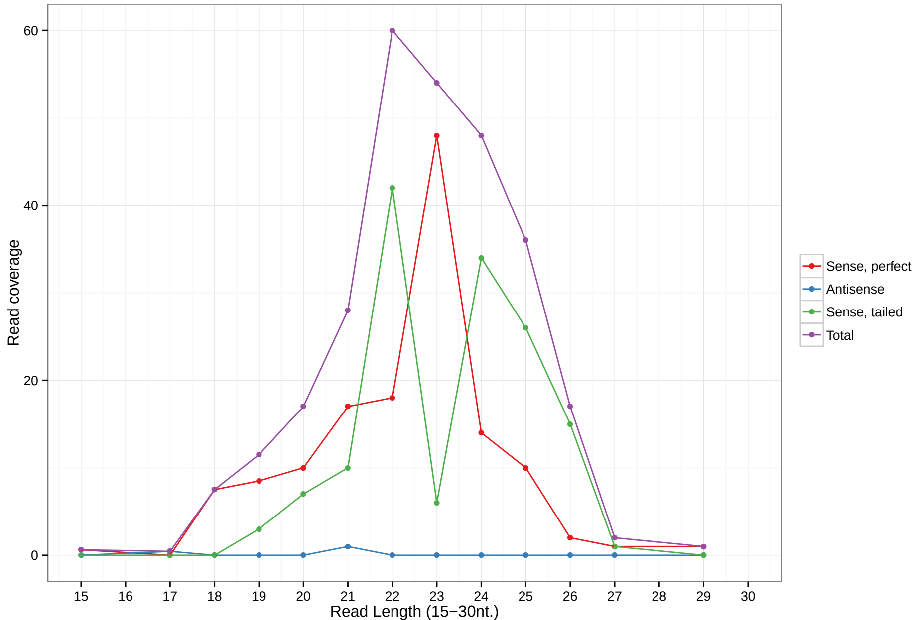
hsa-mir-6751
