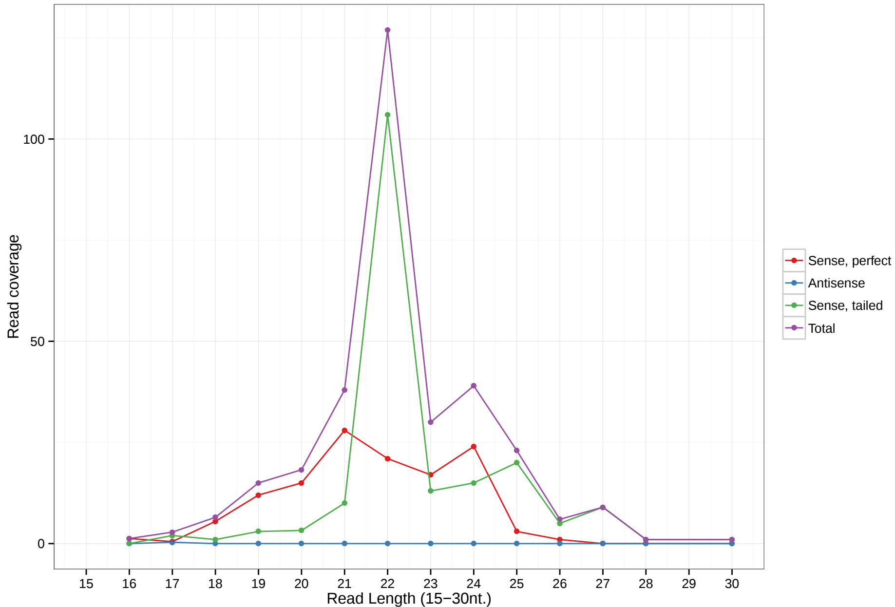
hsa-mir-6750
