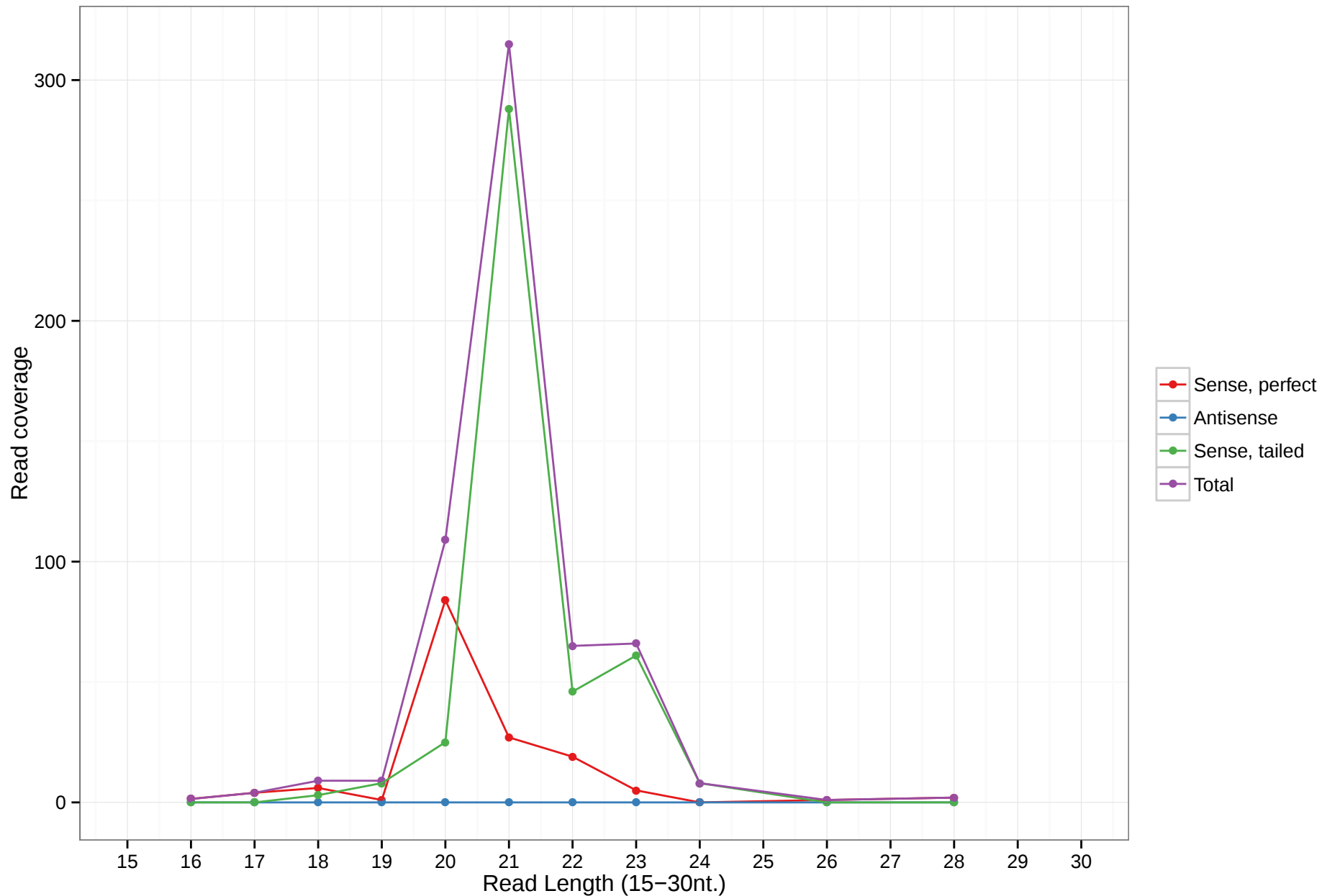
hsa-mir-6742
