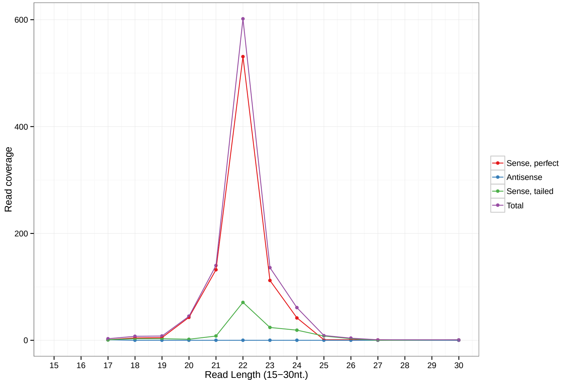
hsa-mir-6716
