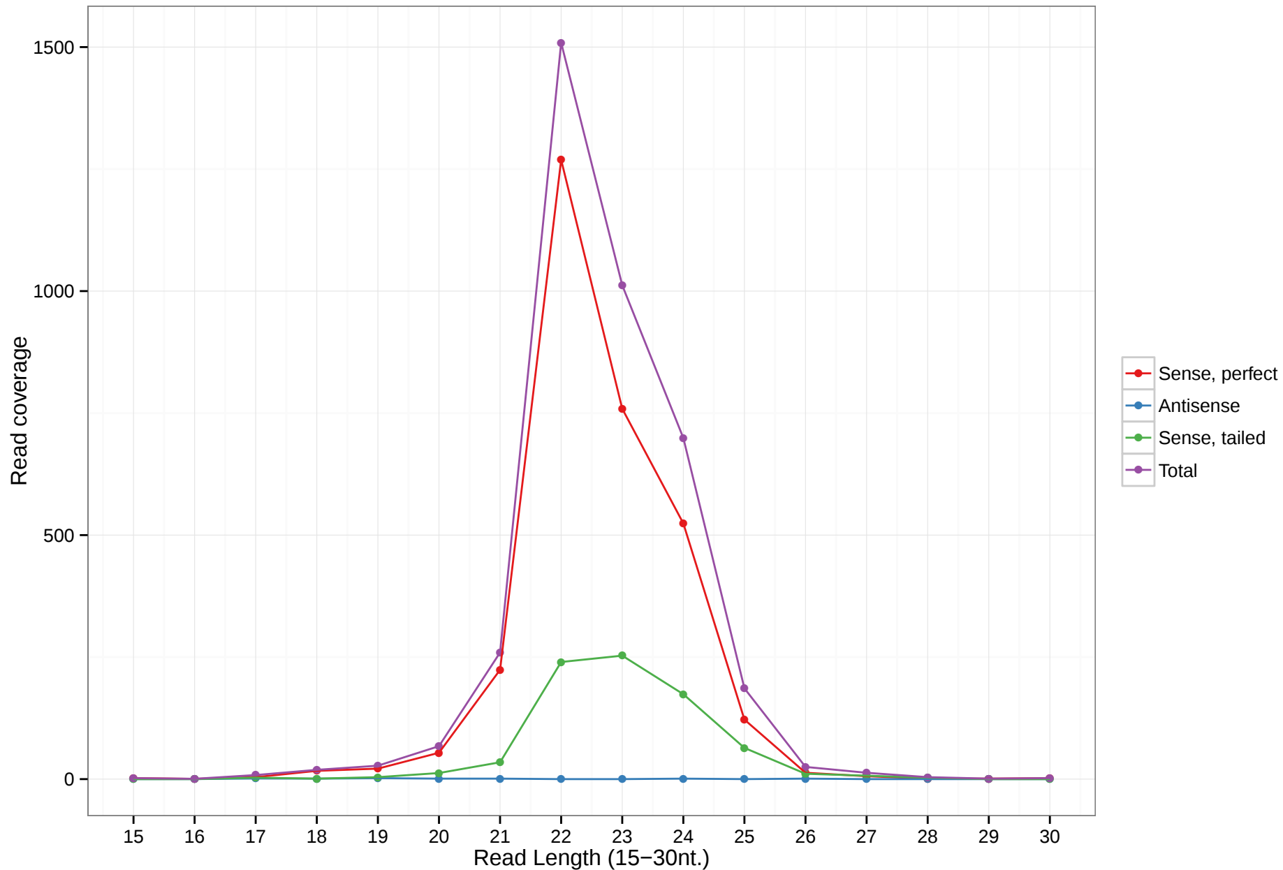
hsa-mir-6514
