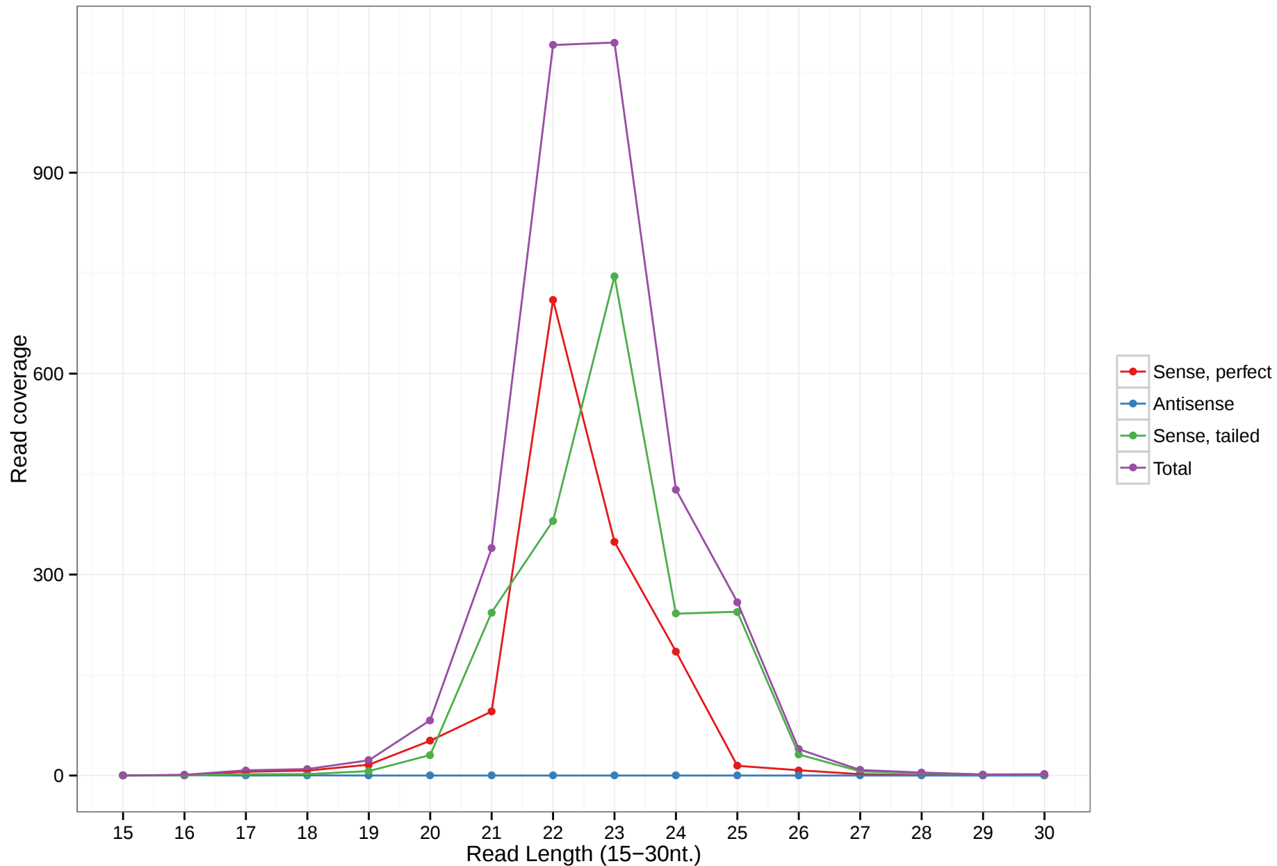
hsa-mir-6511b-2
