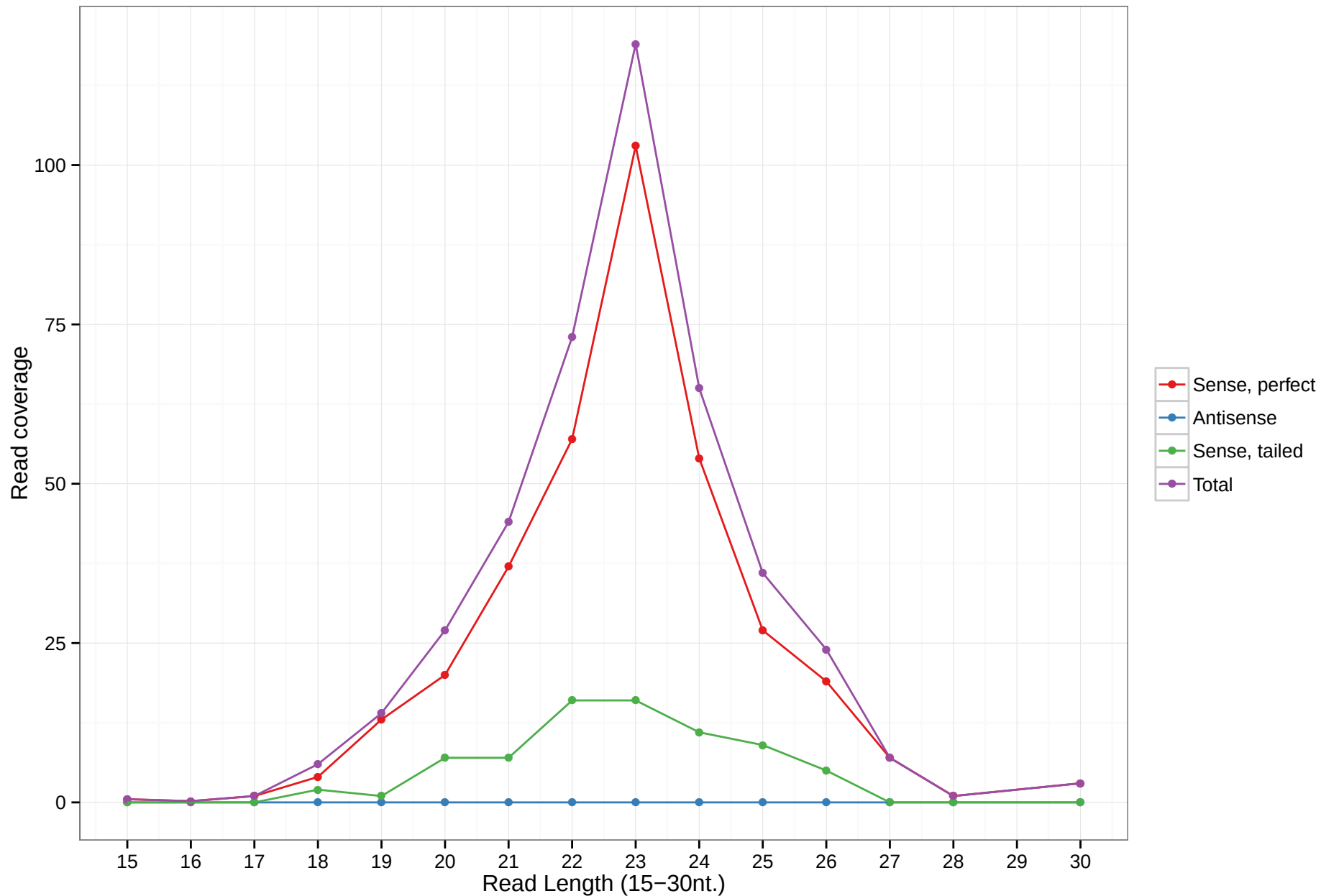
hsa-mir-4723
