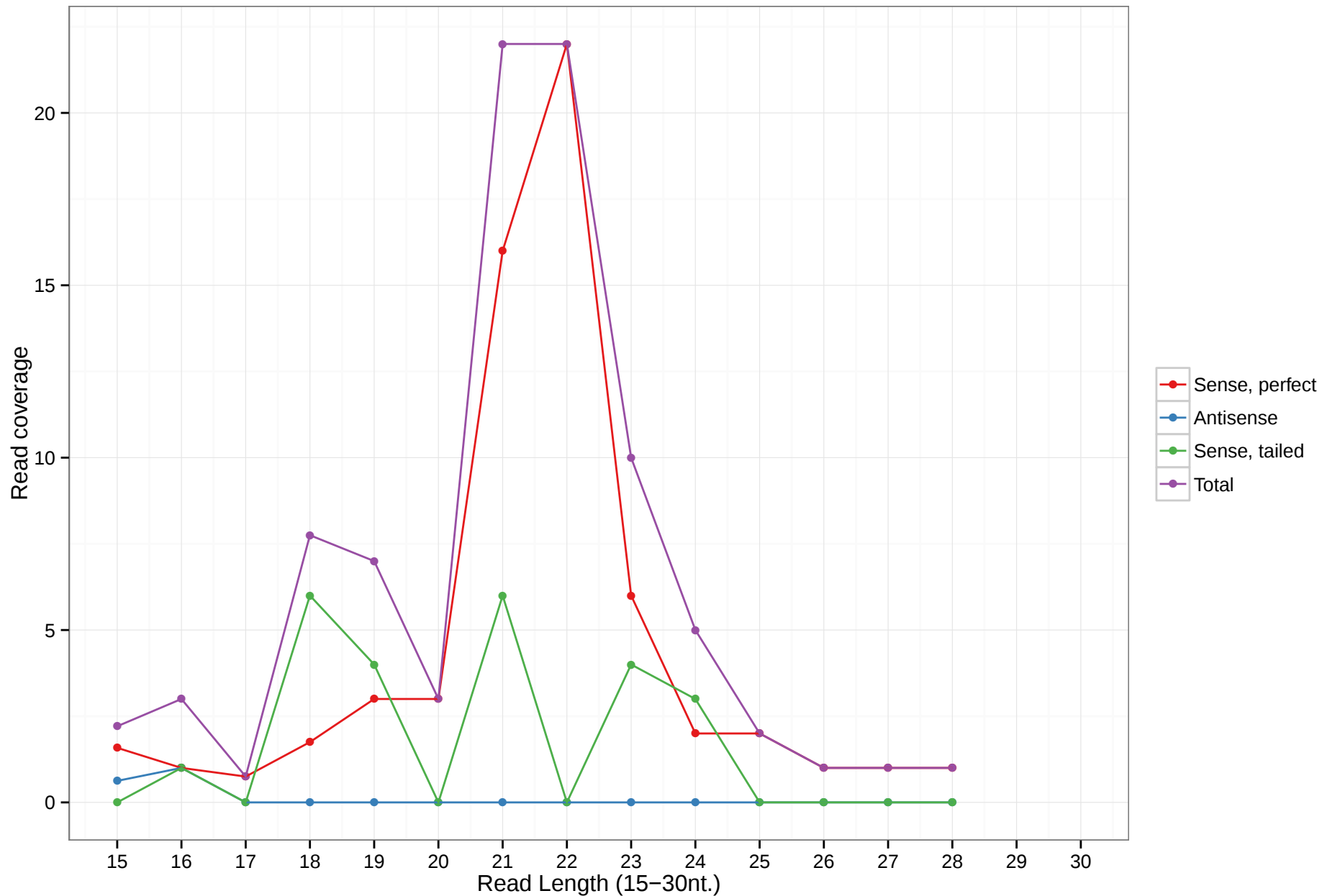
hsa-mir-4673
