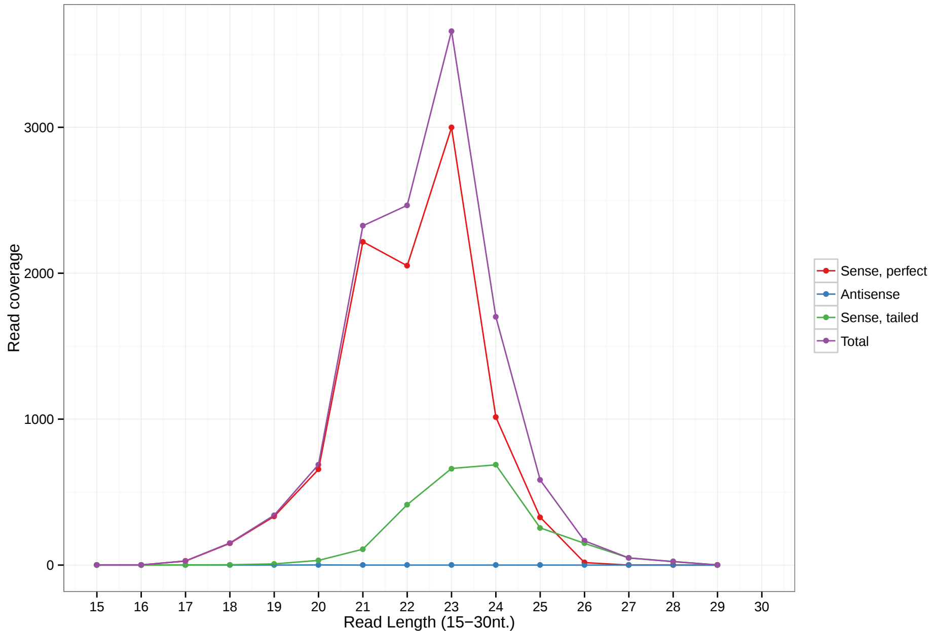
hsa-mir-3605
