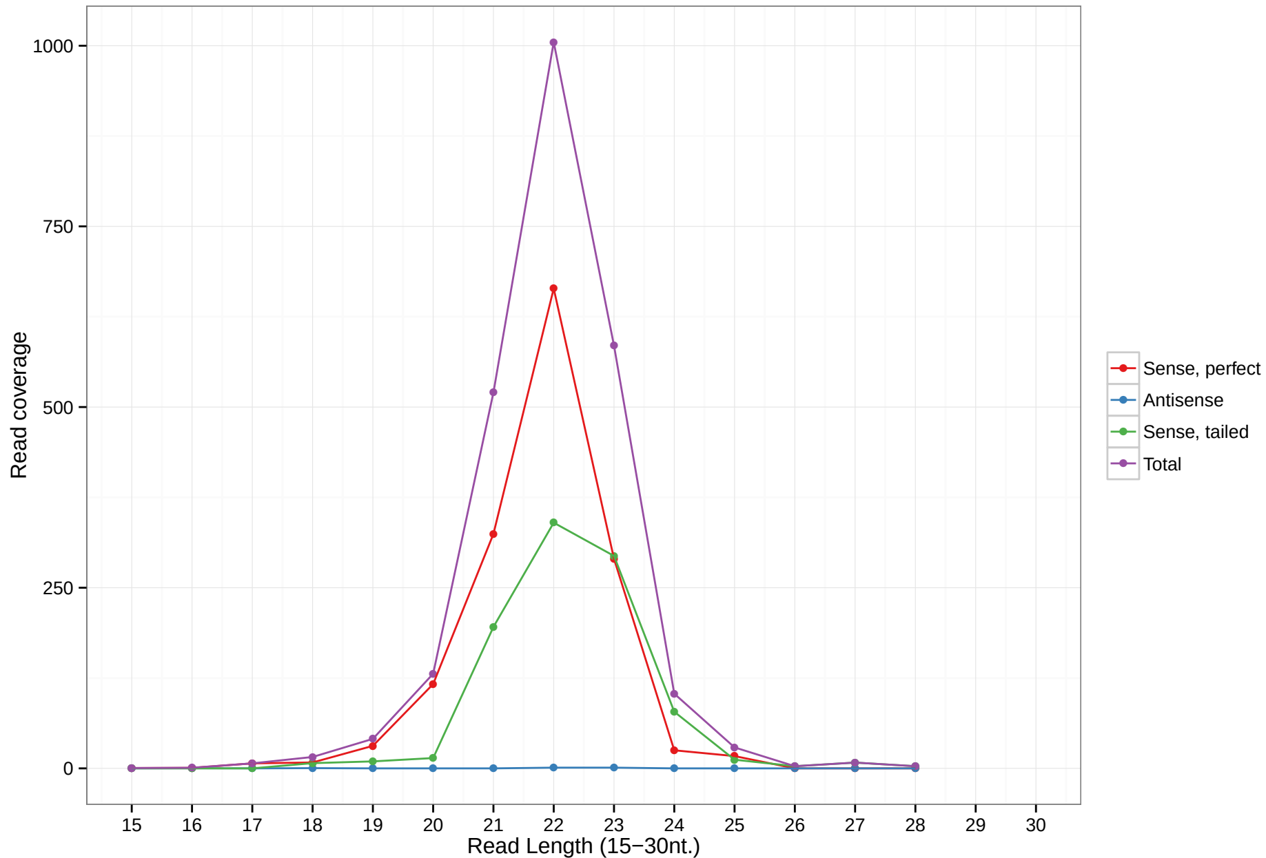
hsa-mir-1976
