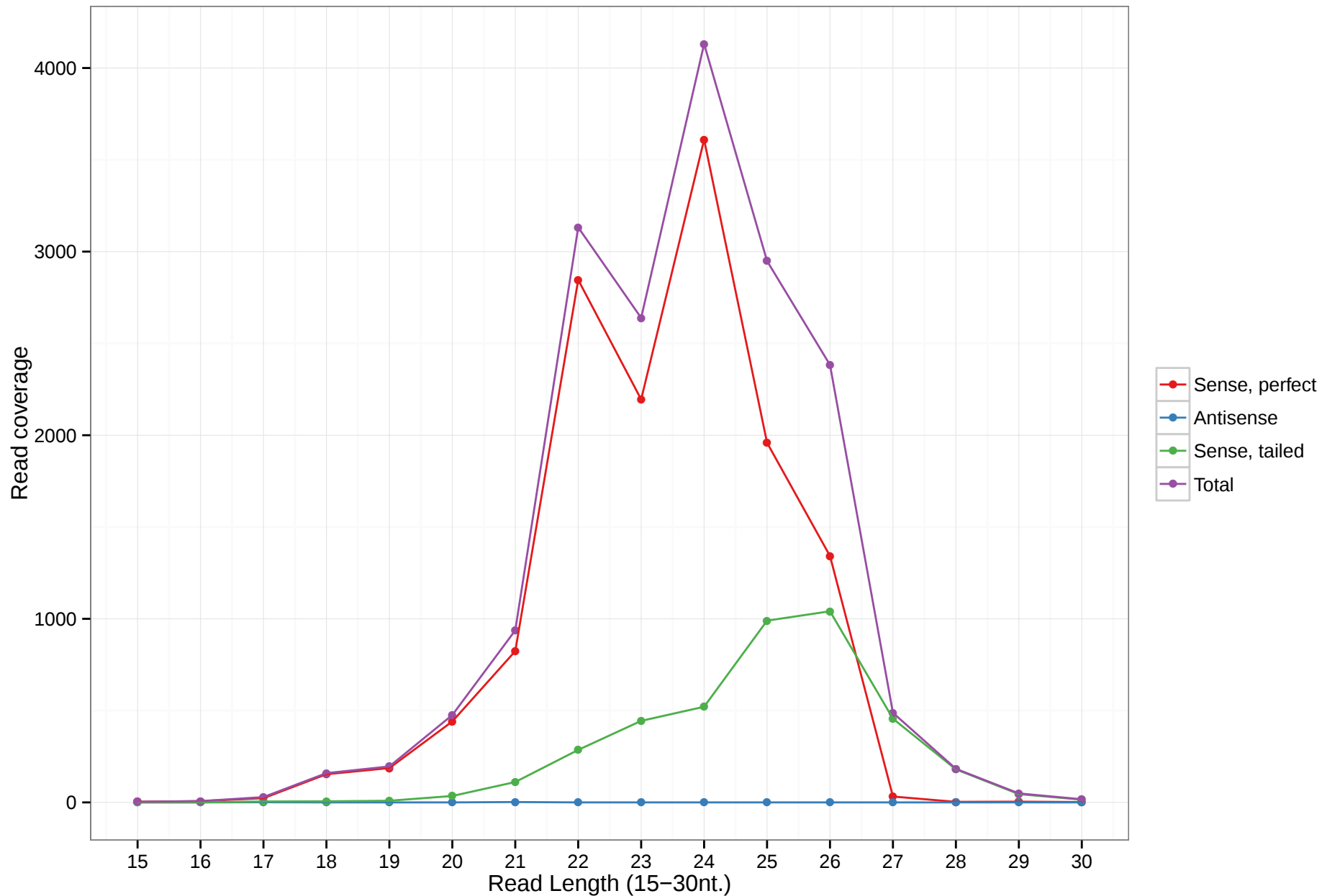
hsa-mir-1292
