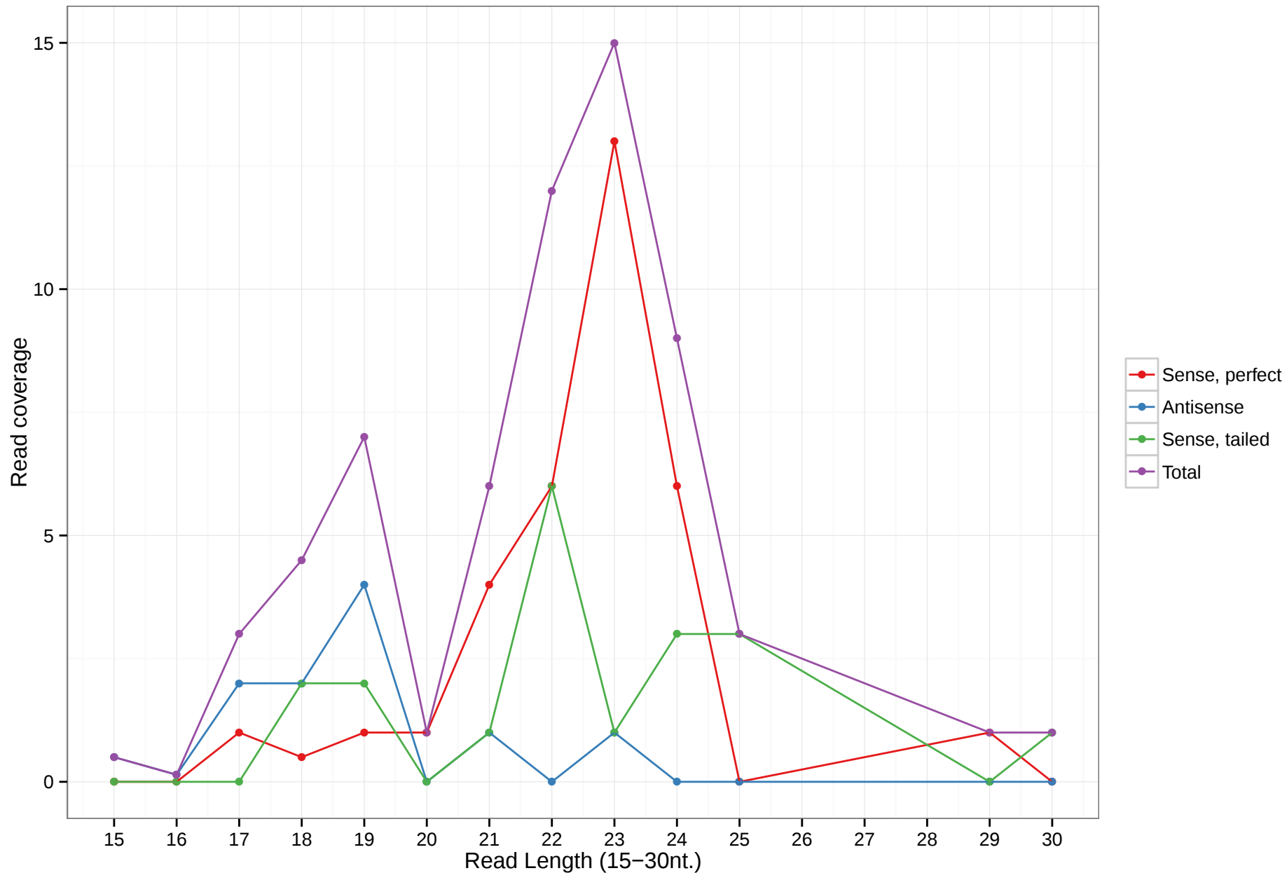
hsa-mir-1238
