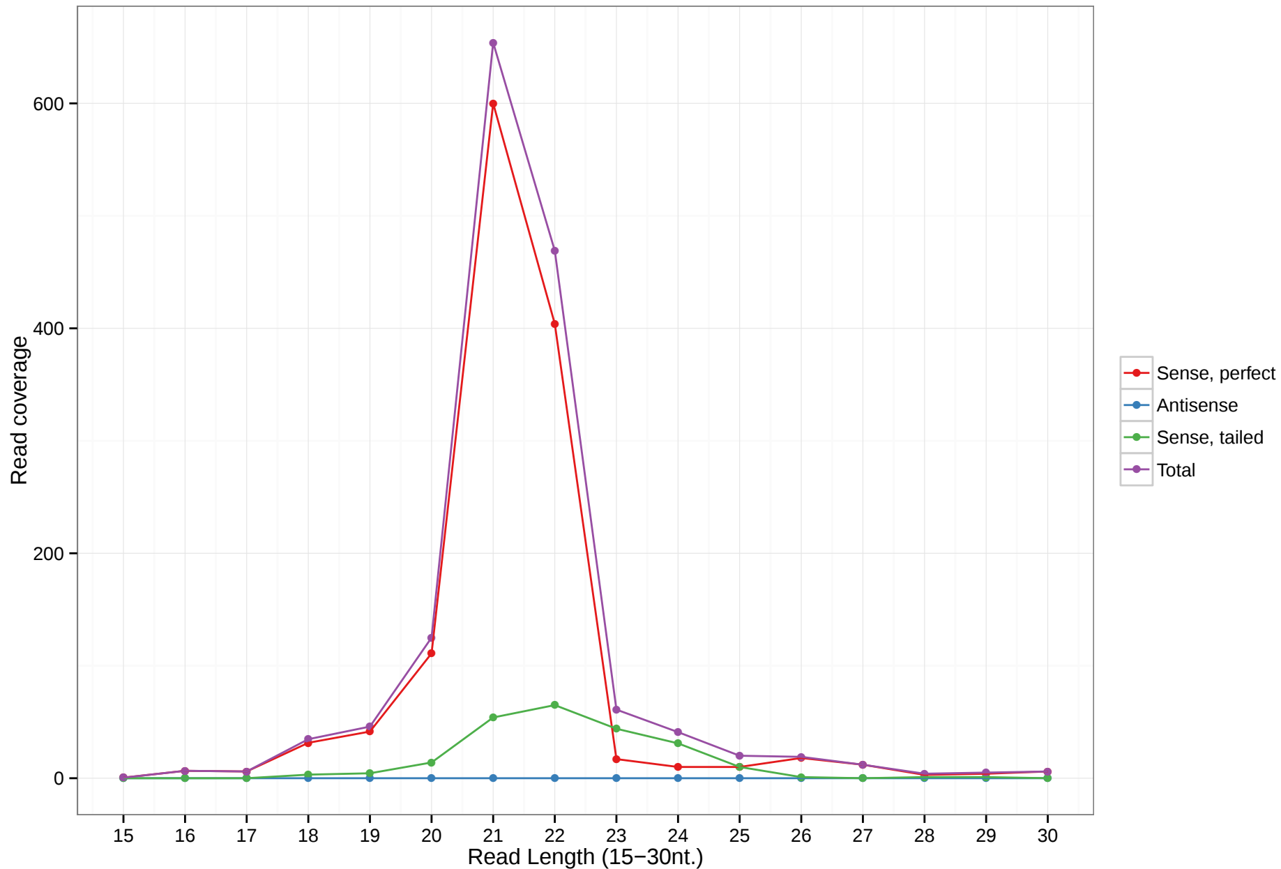
hsa-mir-1228
