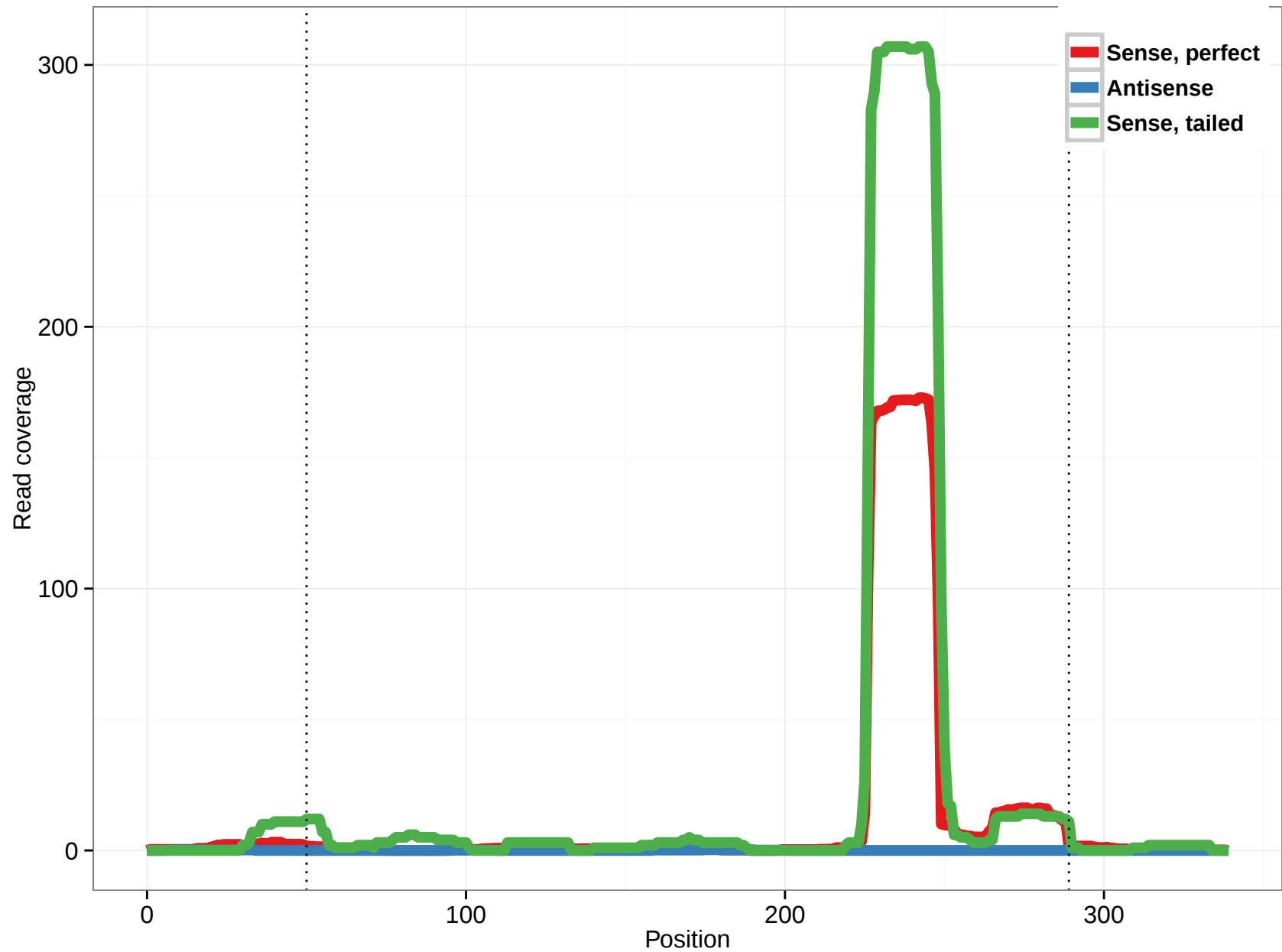
uc010utu.5
