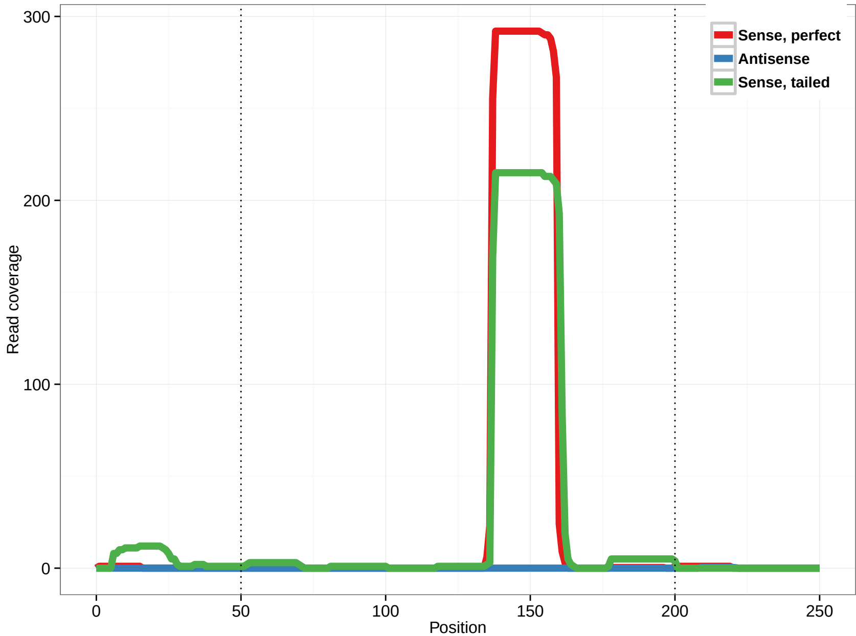
uc001tsa.19
