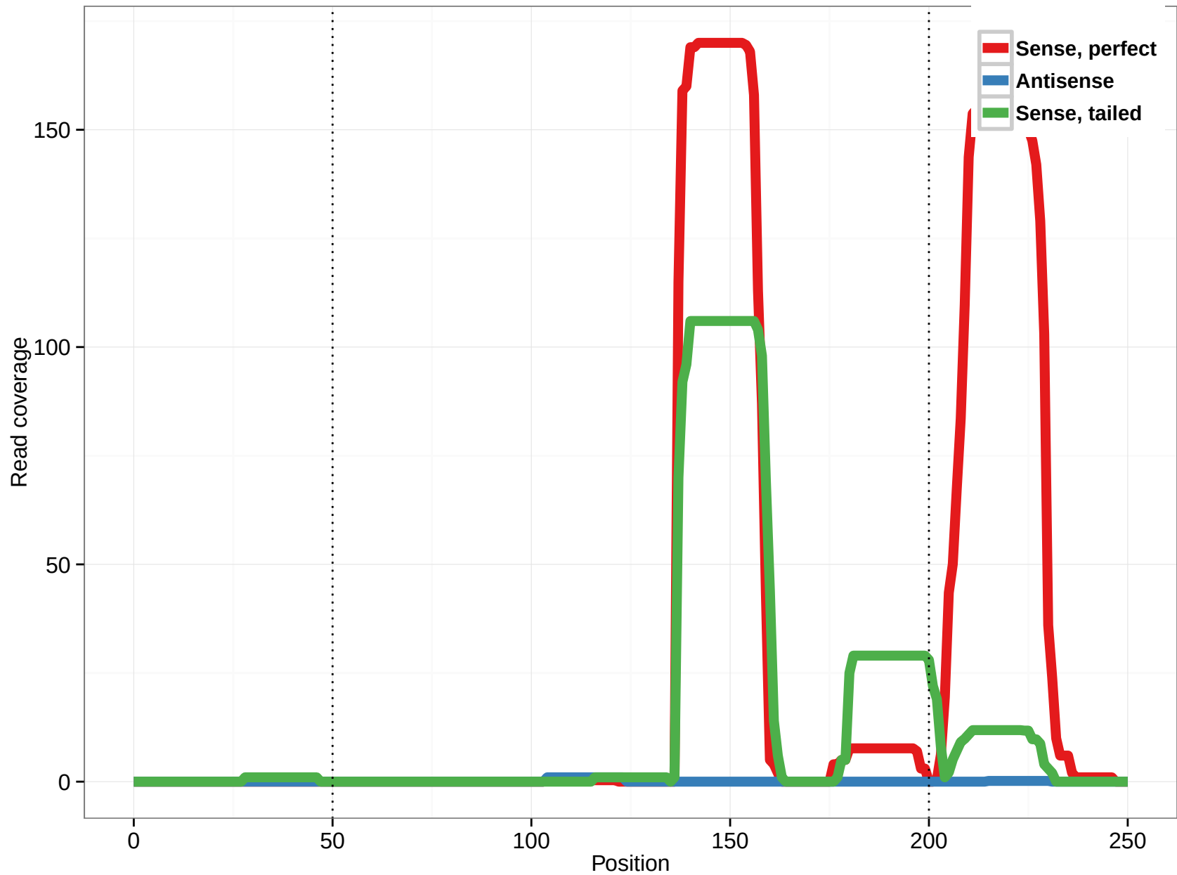
uc001ont.5
