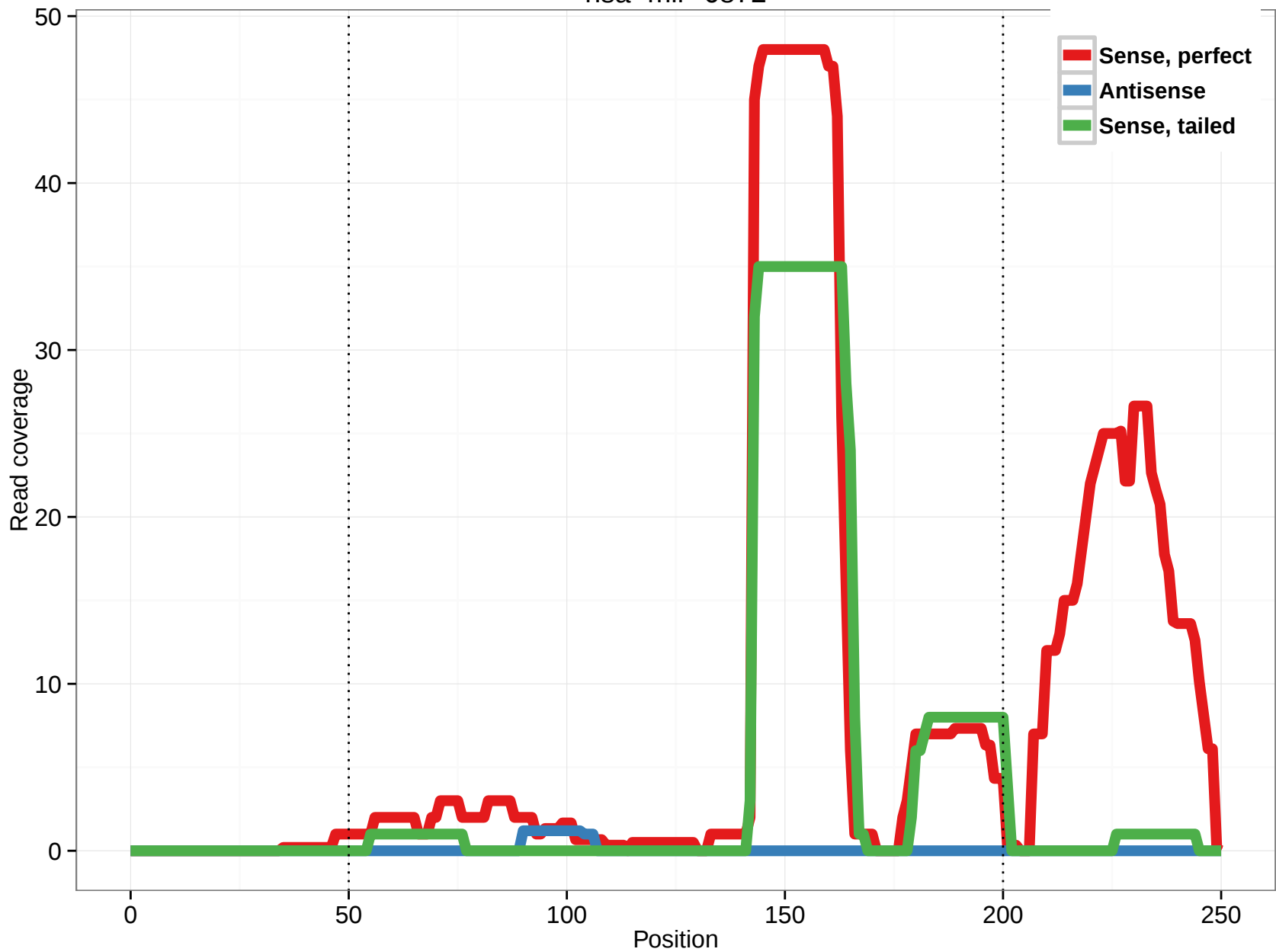
hsa-mir-6872
