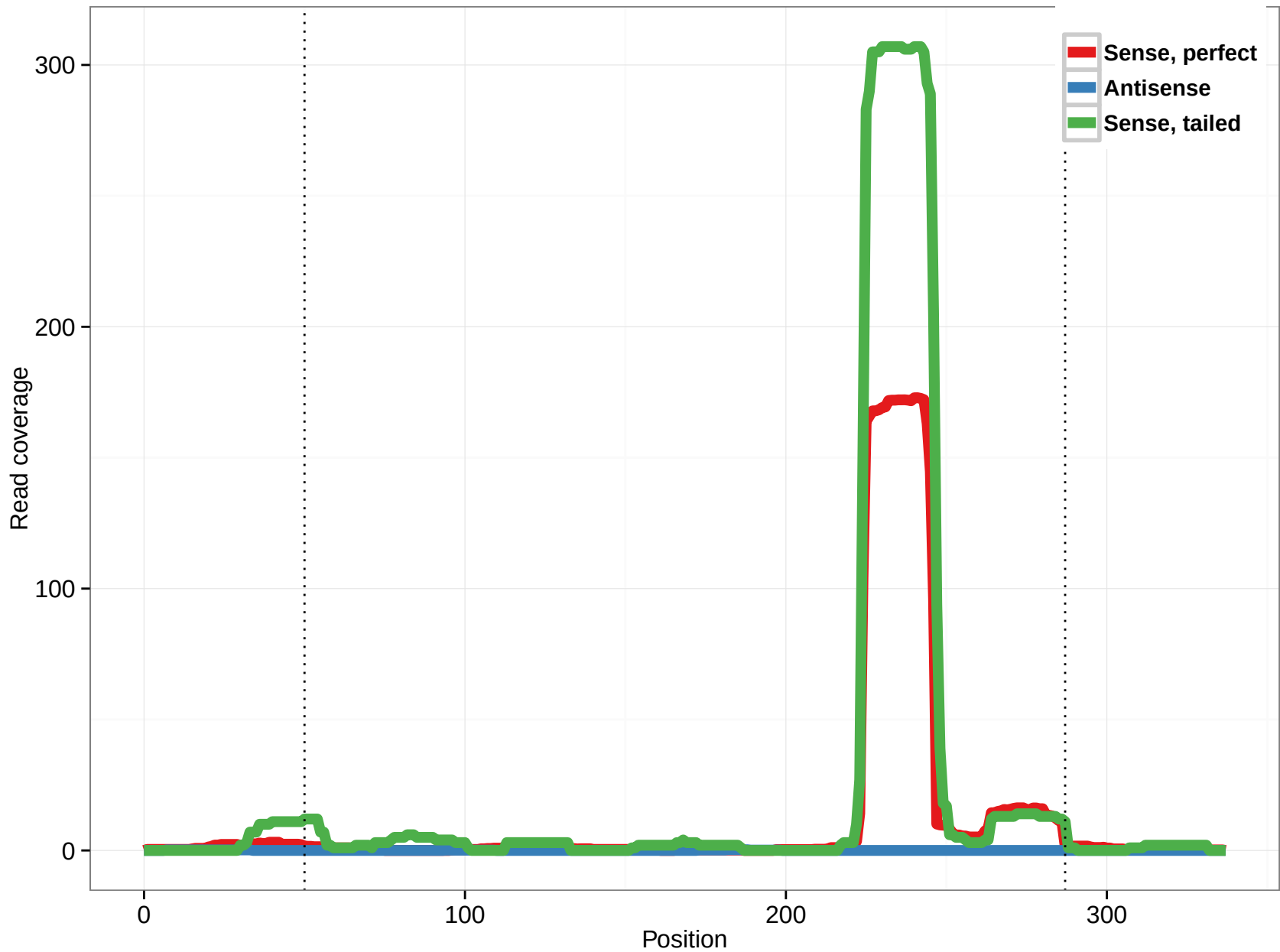
hsa-mir-6859
