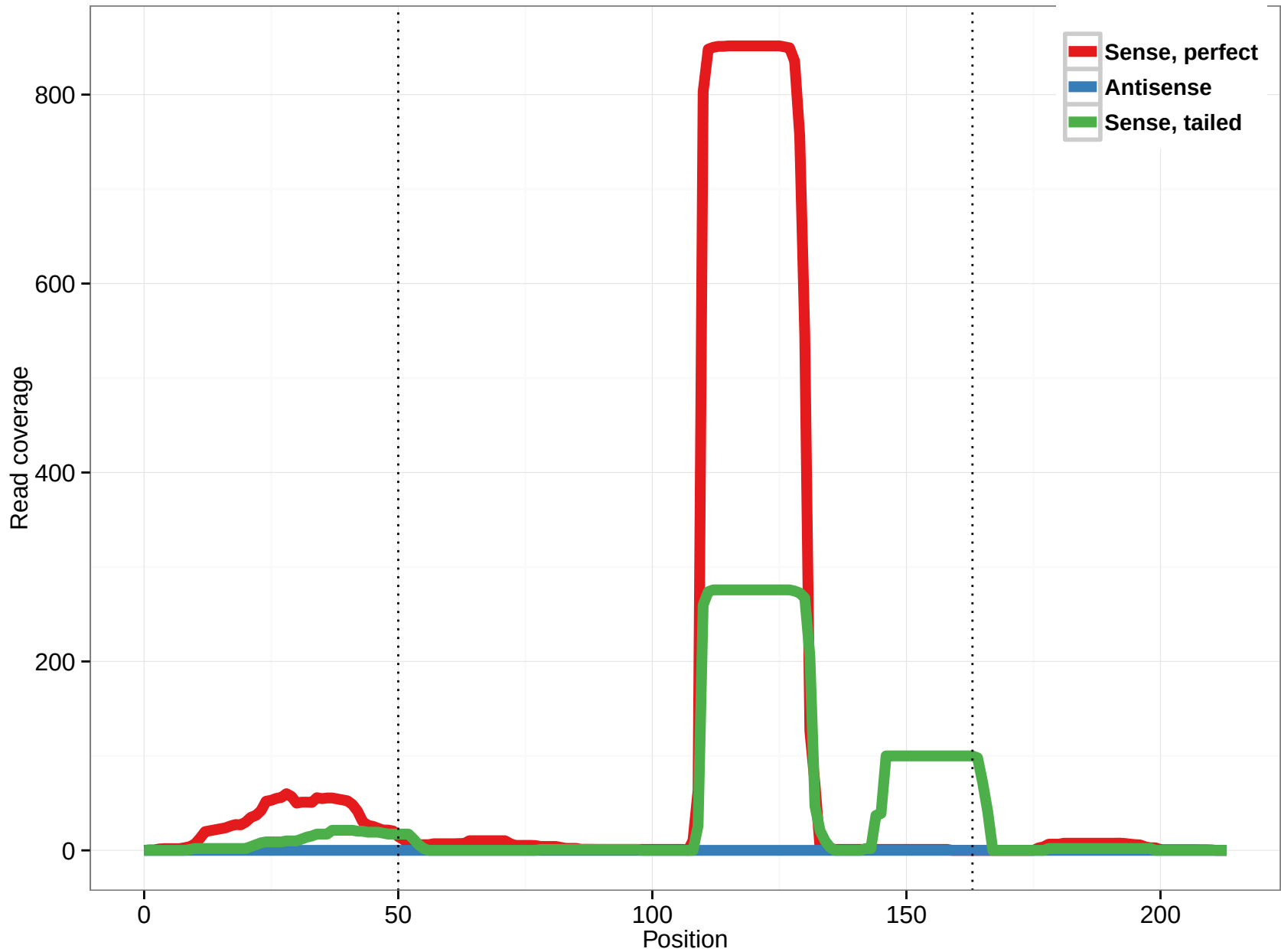
hsa-mir-6852
