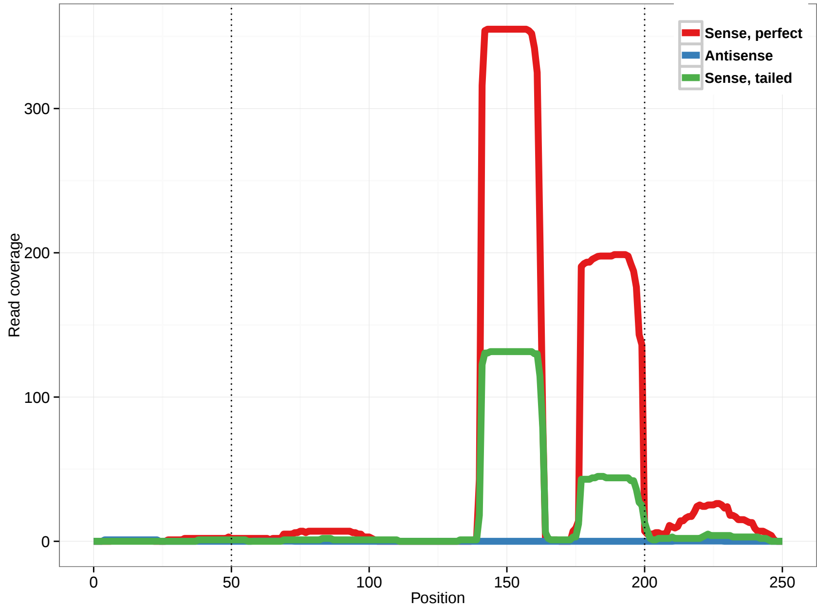
hsa-mir-6837
