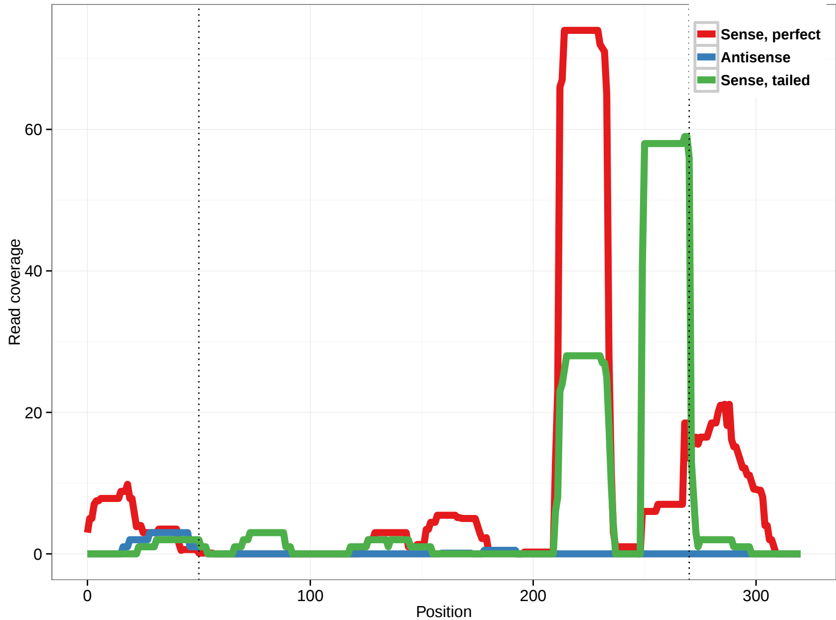
hsa-mir-6836
