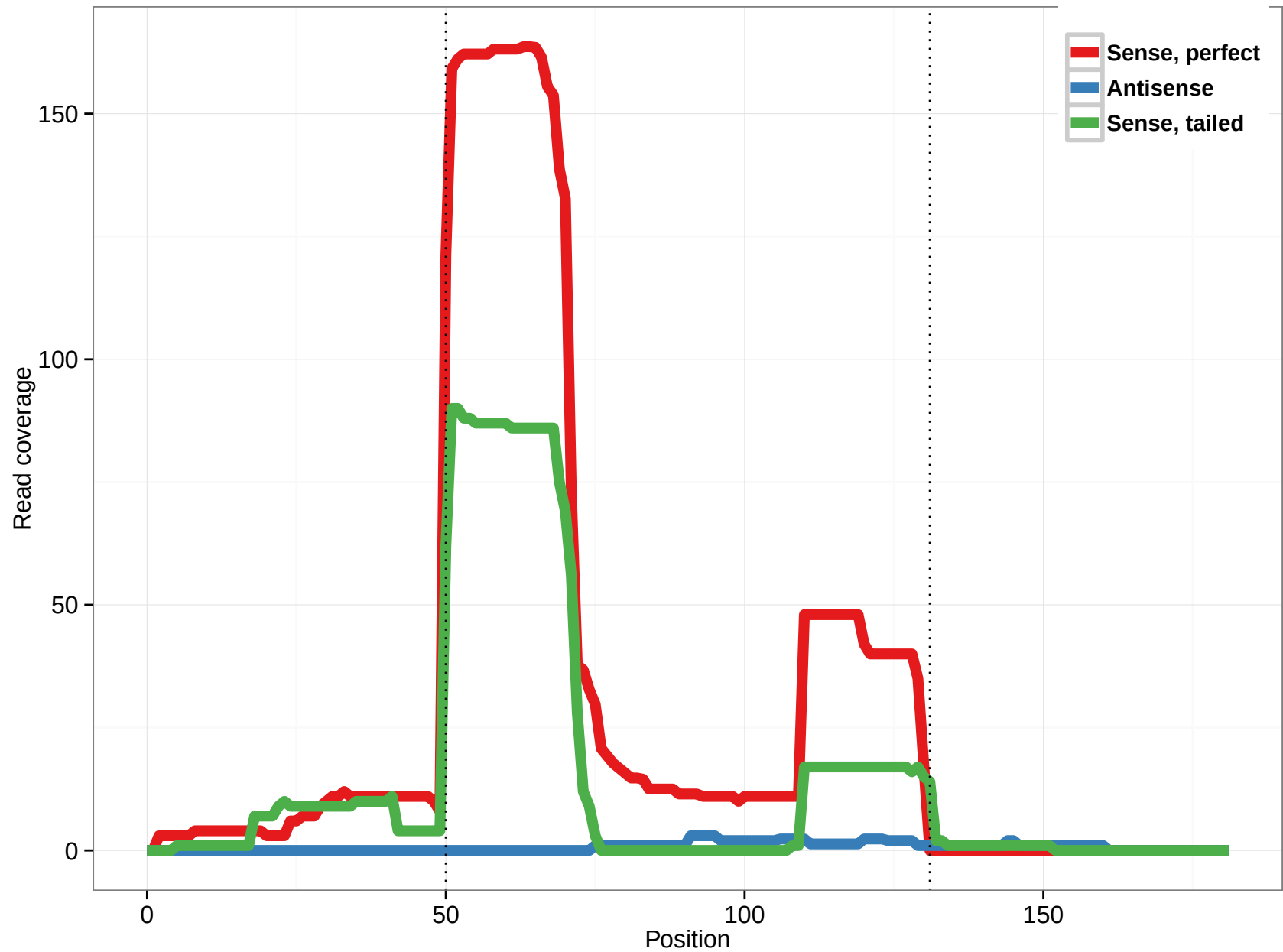
hsa-mir-6834
