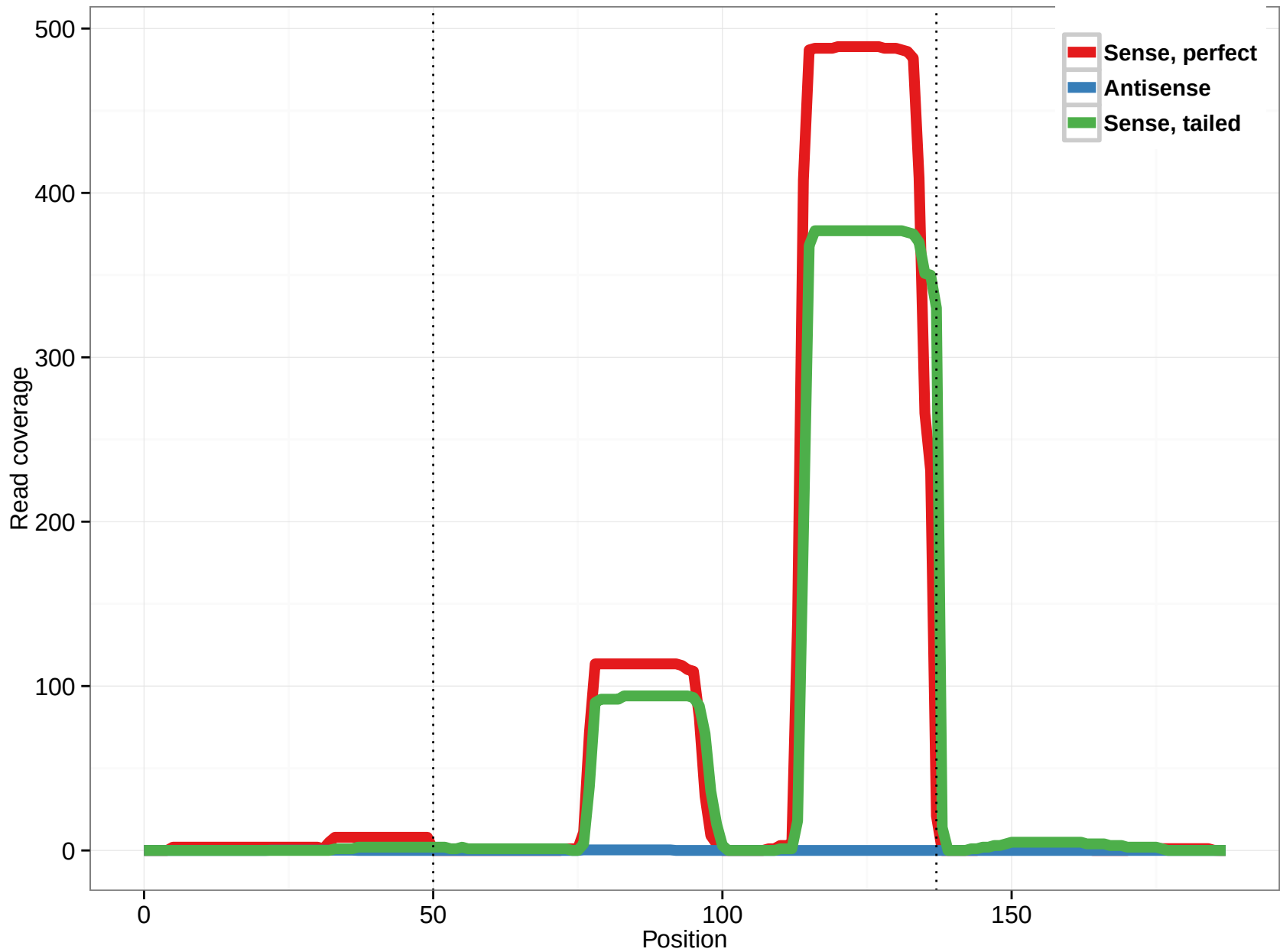
hsa-mir-6802
