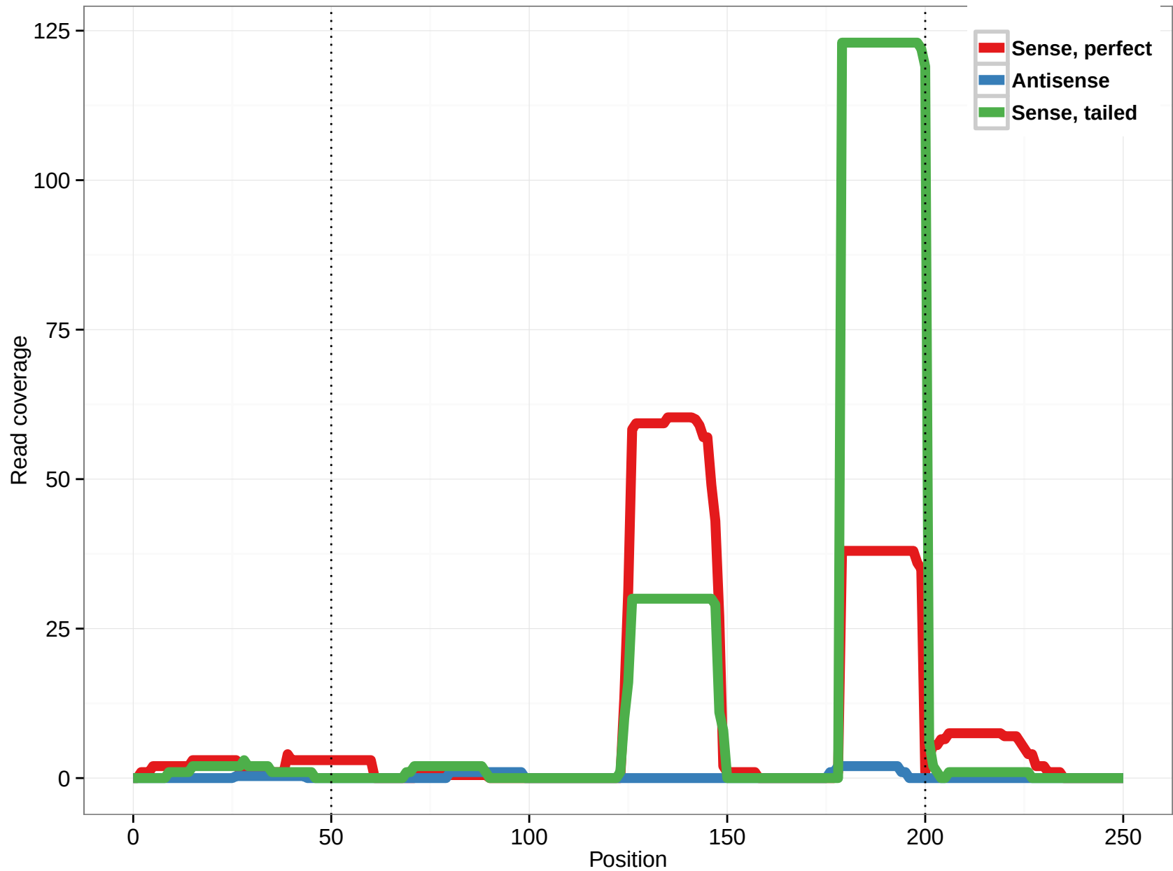
hsa-mir-6780b
