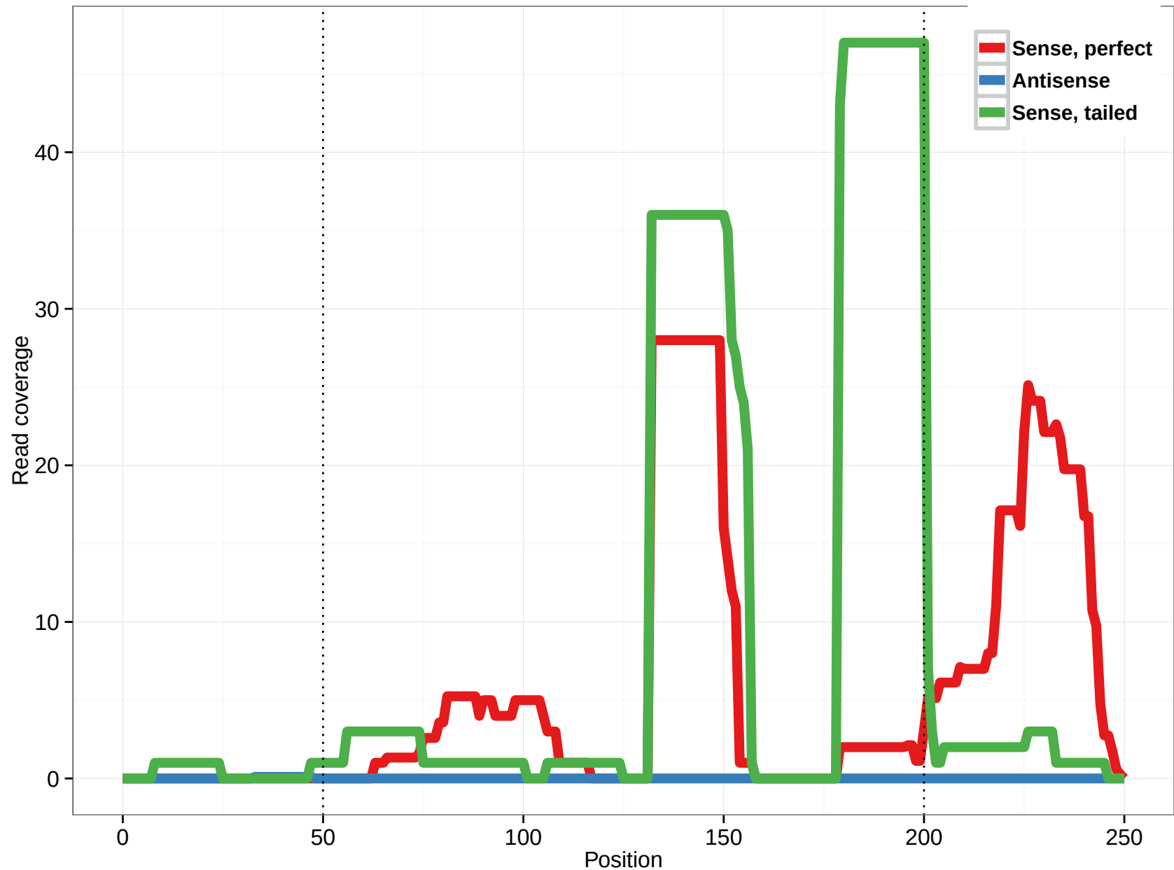
hsa-mir-6769a
