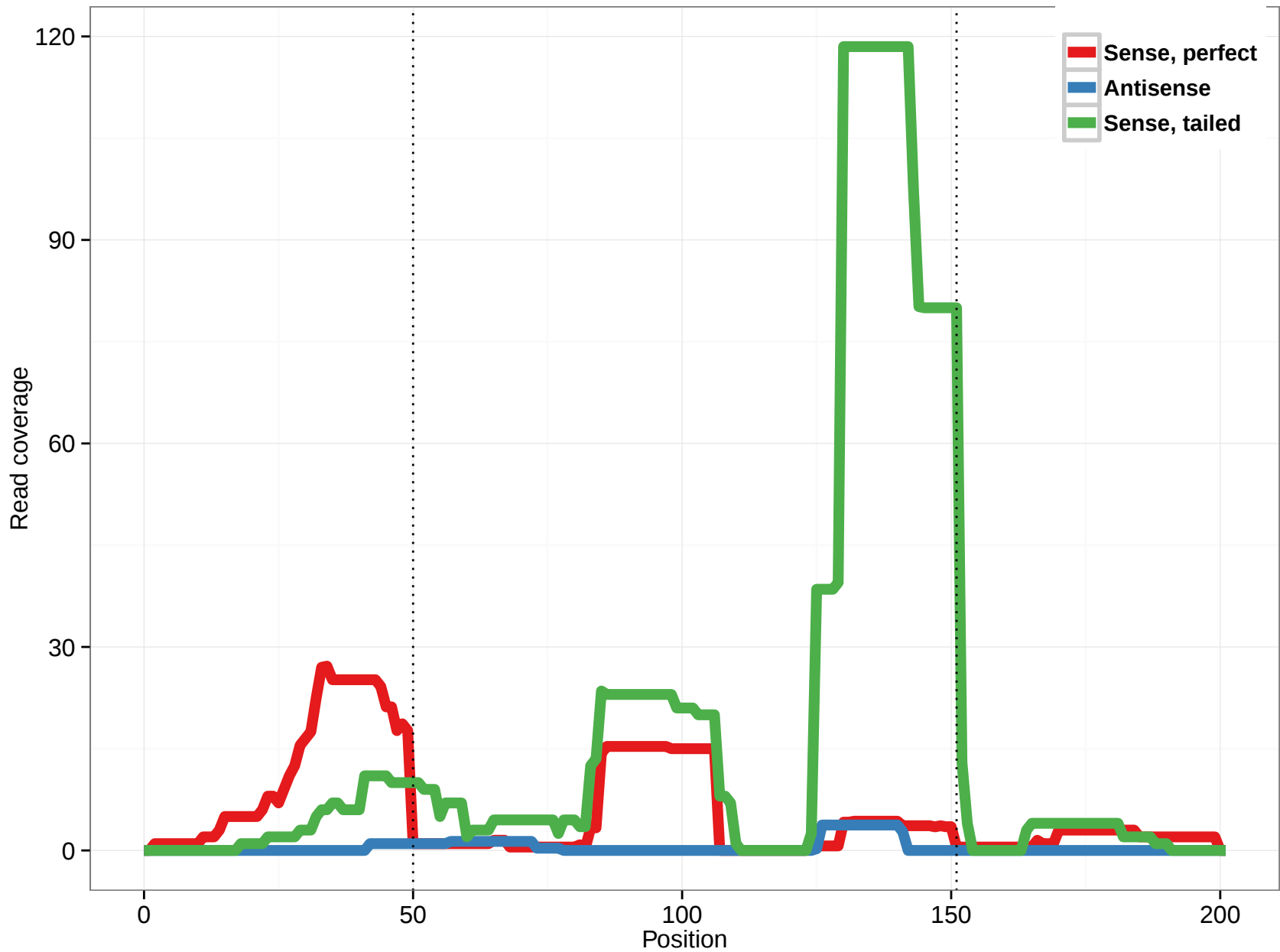
hsa-mir-6752
